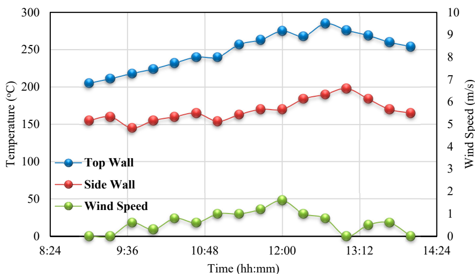
Figure 12. Variation of top wall temperature, sidewall temperature, and wind speed during the experimental day 30 September 2017, with Al_2O_3 /thermal oil nanofluid as the working fluid.
