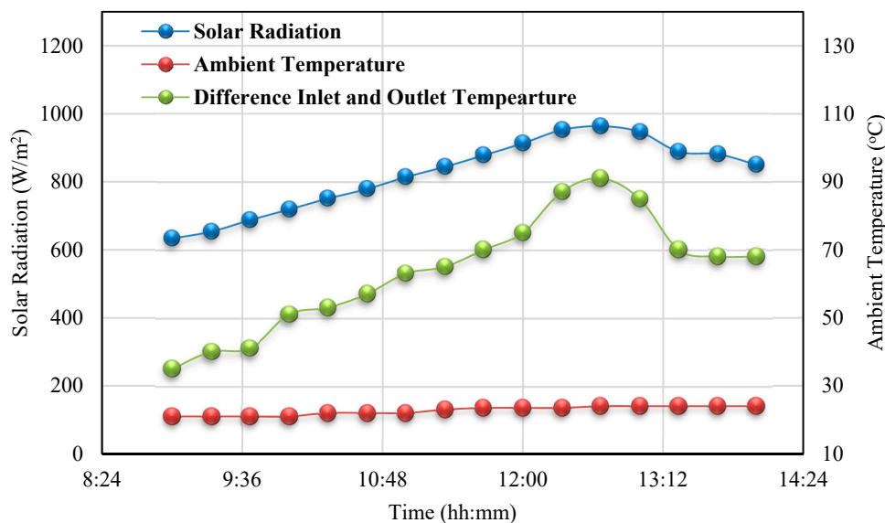
Figure 11. Variation of solar radiation, ambient temperature, and nanofluid temperature difference at the inlet and outlet of the cavity receiver during the experimental day 30 September 2017, with Al_2O_3 /thermal oil nanofluid as the working fluid.
