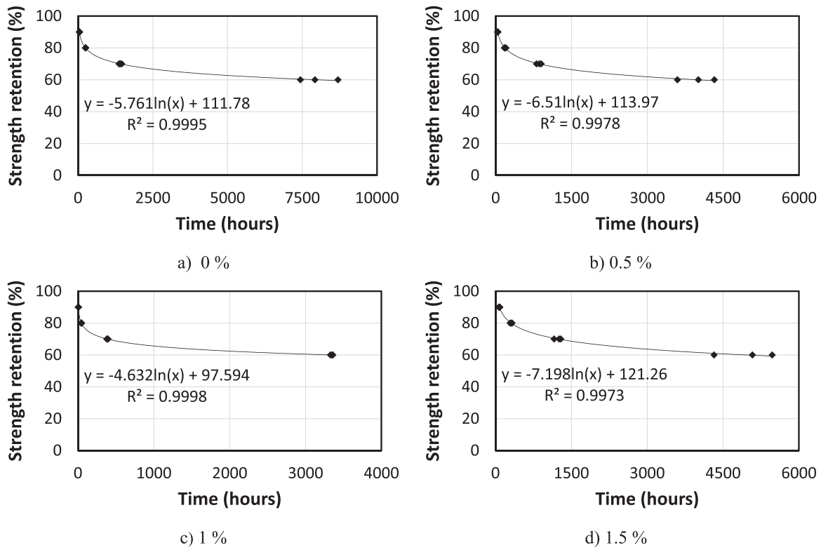
Fig. 15. : Master cures for ILSS retention of hybrid composites at 20 °C.
