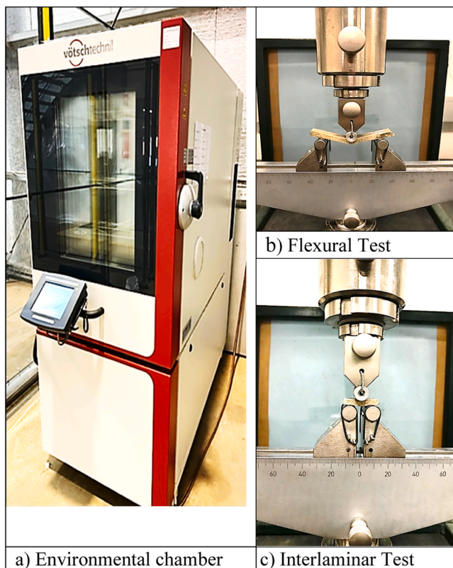
Fig. 2. : Aging and mechanical tests for hybrid composites.
