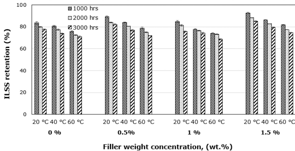
Fig. 9. : ILSS retention of hybrid composites under hygrothermal conditioning.
