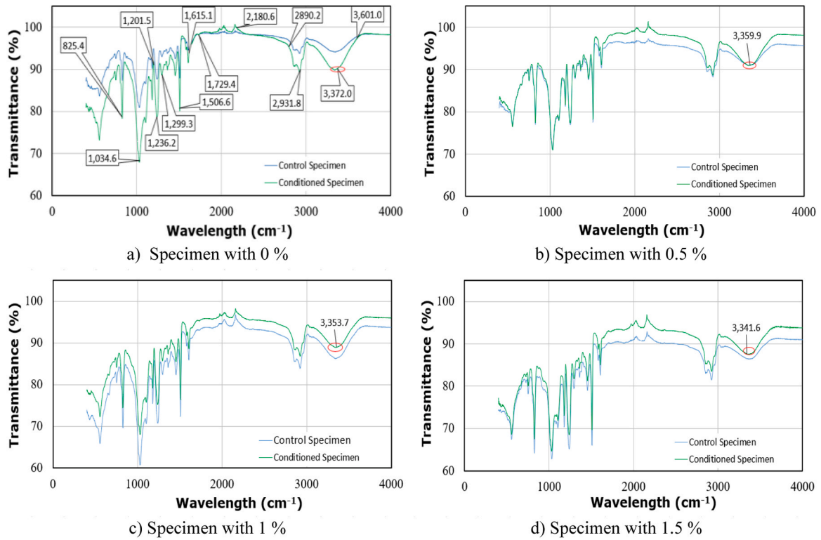
Fig. 11. : FTIR spectra of hybrid composites.
