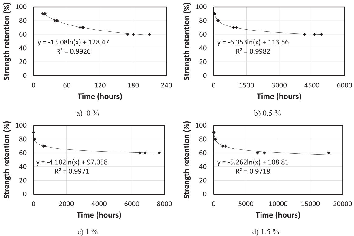
Fig. 16. : Master cures for FS retention of hybrid composites at 30 °C.
