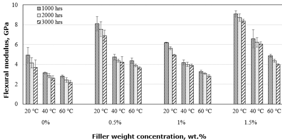
Fig. 6. : Flexural modulus of hybrid composites under hygrothermal conditioning.
