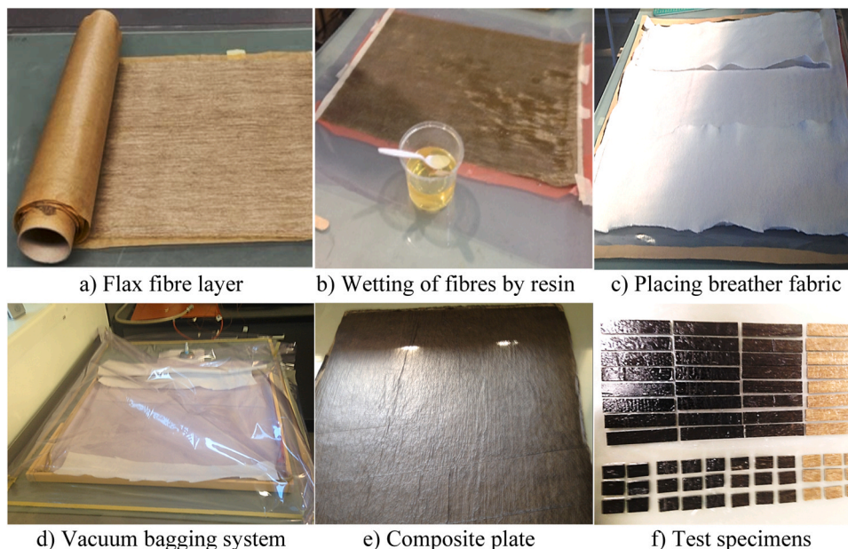
Fig. 1. Manufacturing process for hybrid composite laminates.
