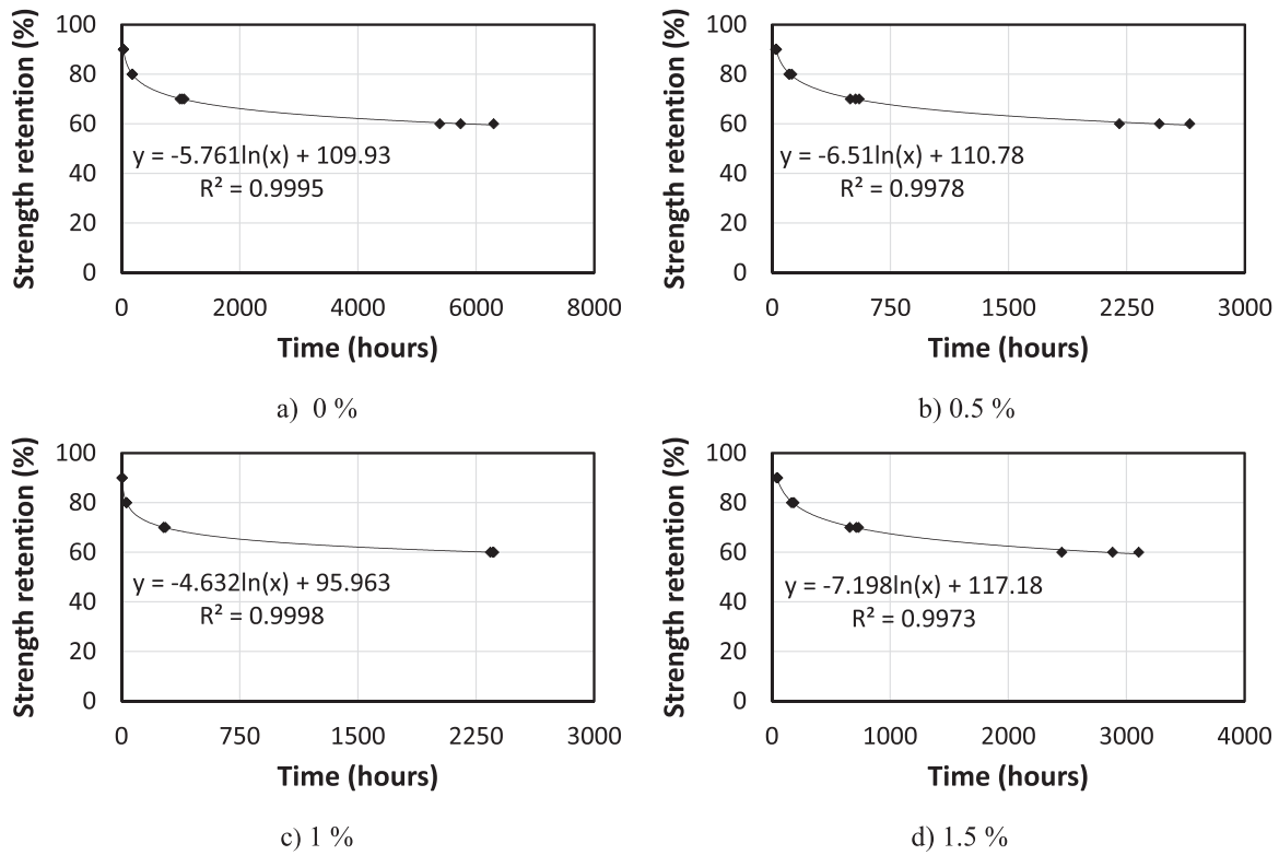
Fig. 17. : Master cures for ILSS retention of hybrid composites at 30 °C.
