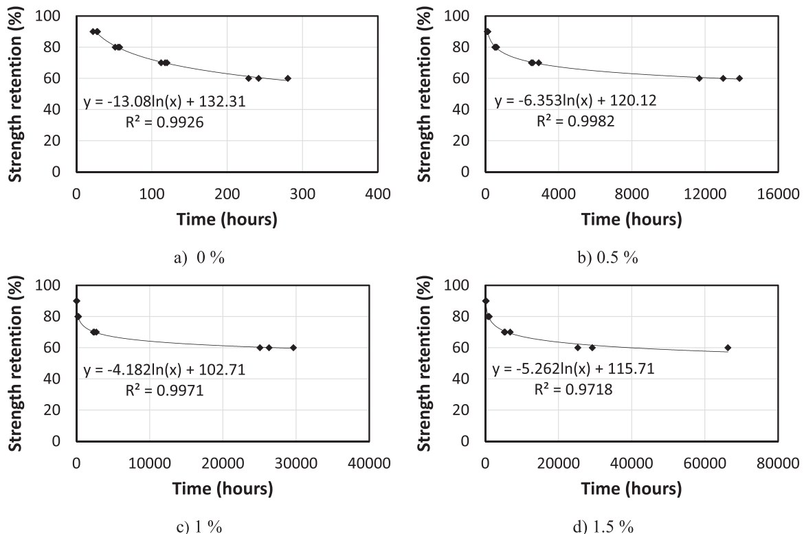
Fig. 14. : Master cures for FS retention of hybrid composites at 20 °C.
