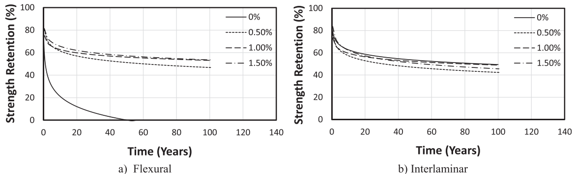
Fig. 18. : Service life of hybrid composites at 30 °C.
