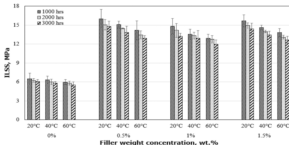
Fig. 8. : Interlaminar shear strength of hybrid composites under hygrothermal conditioning.
