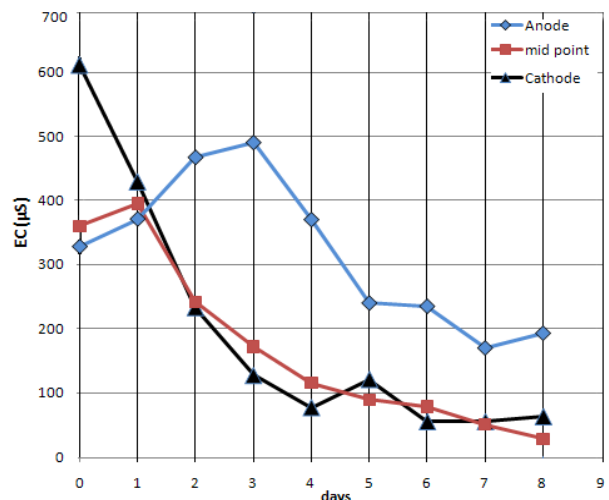
Figure 7 Electrical conductivity of extracted soil-water when applying voltage gradient 3 \text{Vcm}^{-1}
