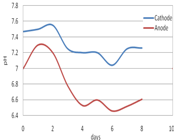
Figure 8 Soil pH when applying electrical gradient of 3Vcm^{-1}
