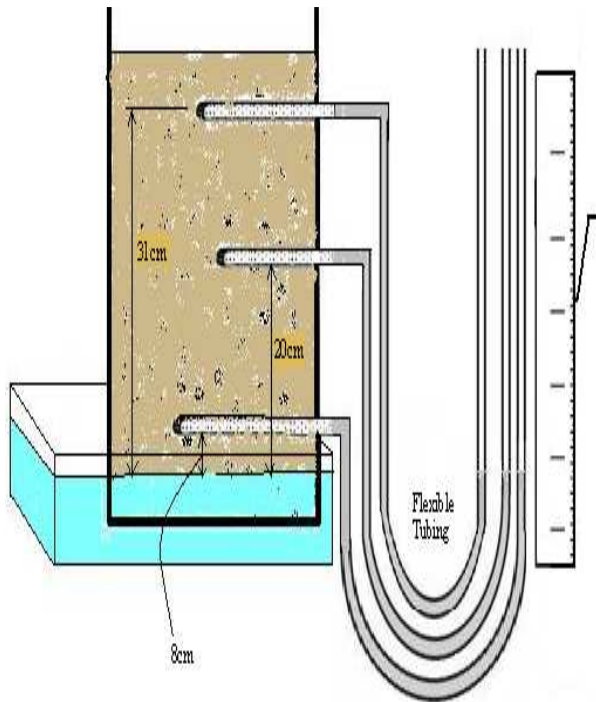
Figure 4 Schematic of hanging water column technique
