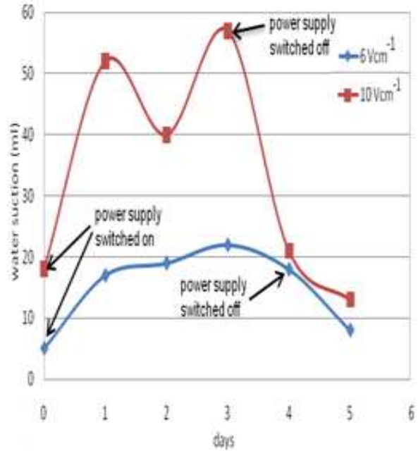
Figure 3 Volume of water extracted from top lysimeter when applying electrical gradients of 6 & 10\text{Vcm}^{-1}
