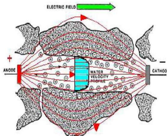
Figure 1 Principle of electro-osmosis through soil capillary.
