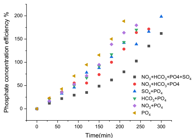
Fig. 11. Effect of different ions on the phosphate concentration efficiency over operating time.
