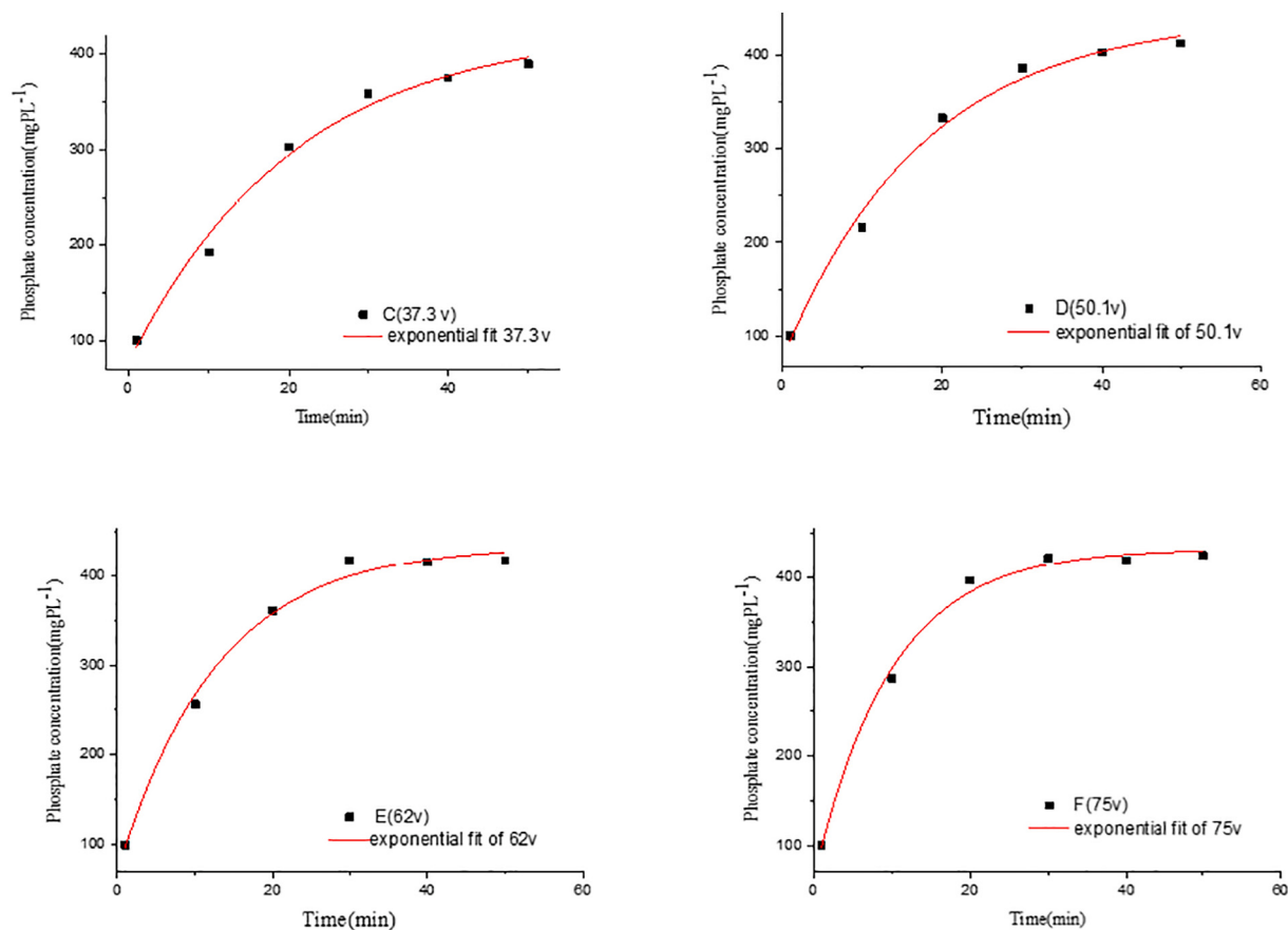
Fig. 8. Regression between phosphate concentration in respect to the operating time for different voltages (data from Wang et al. [29]). The markers represent experimental values while the solid lines represent the fitted equations.
