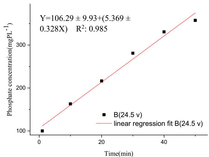
Fig. 7. Linear regression between phosphate concentration with respect to the operating time in 24.5 v (data from Wang et al. [29]). The markers represent experimental values, while the solid lines represent the fitted equation.
