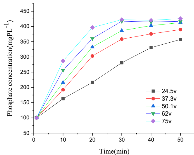
Fig. 6. Effect of voltage on phosphate concentration over operating time. (Data from Wang et al. [29].)
