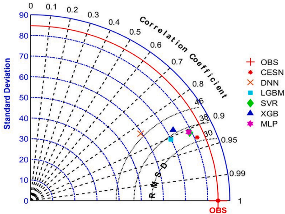
Fig. 14. Taylor diagram depicting the correlation coefficient, standard deviation and root mean square deviation ( RMSD ) of CESN vs. DNN, LGBM, SVR, XGB and MLP models. (For interpretation of the references to color in this figure legend, the reader is referred to the web version of this article.)
