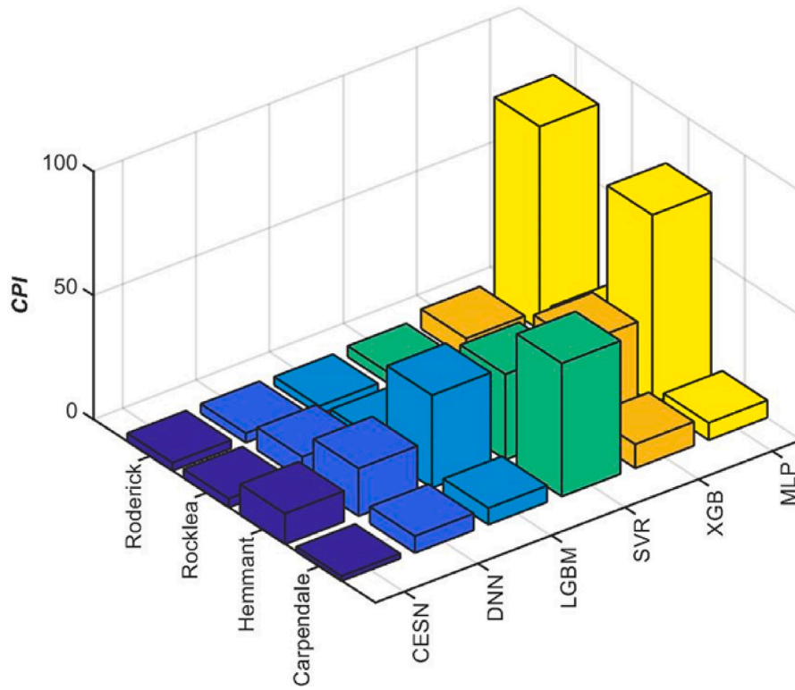
Fig. 13. 3D-bar plot of the Combined Performance Index ( CPI ) of CESN vs. the comparative DNN, LGBM, SVR, XGB and MLP models used in prediction of daily electricity demand ( G ). Names for each model are provided in Table 3.
