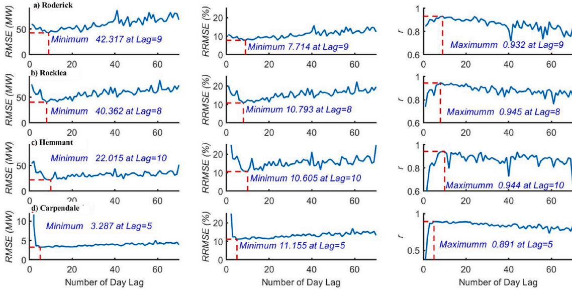
Fig. 6(b). Lag period optimization for daily electricity prediction based on RMSE (MW), RRMSE (%) and correlation coefficient r for all substations.
