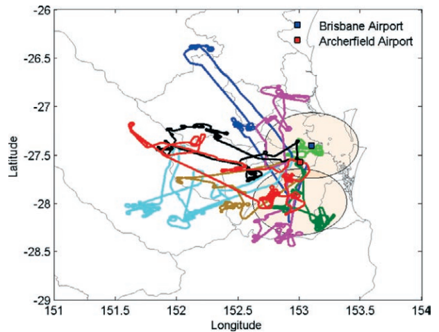
FIG. 3. Map of various flight tracks (each indicated by a different color) around the Brisbane region. The dual-Doppler lobes (from Fig. 1) are overlaid, and the Archerfield and Brisbane airports are highlighted for reference. Faint gray lines indicate the watershed boundaries in the region.
