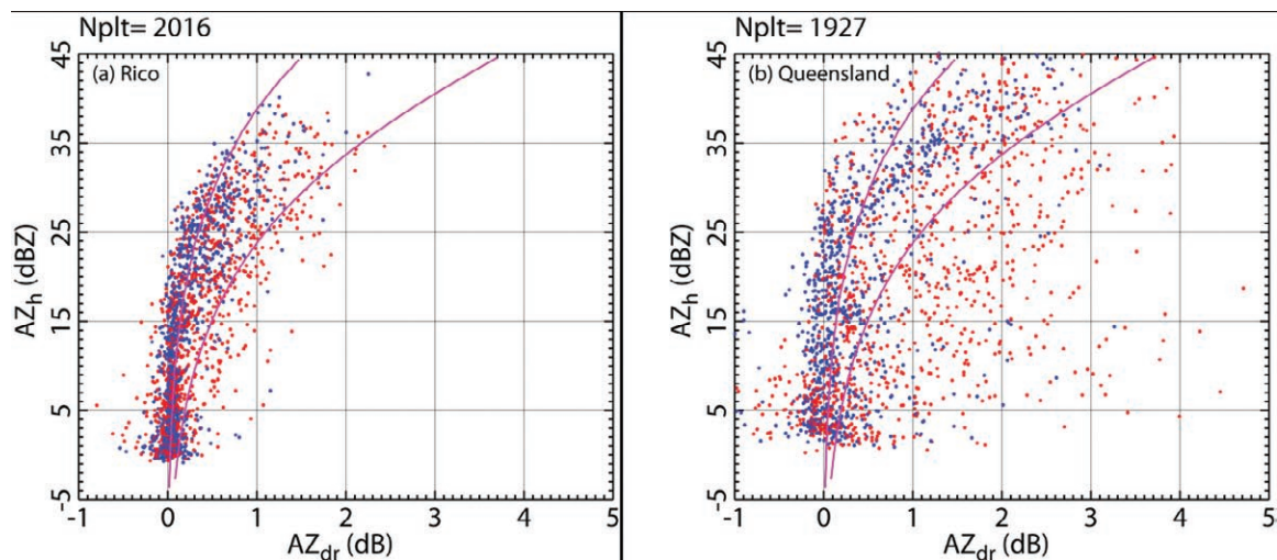
FIG. 7. Scatter plots of AZ_h versus AZ_{dr} for (a) the maritime Caribbean environment from RICO (190 clouds) and (b) Queensland from the QC-SRP (30 clouds). The letter A is used to signify that the individual points represent area Z_h and Z_{dr} values that are calculated for the whole sweep (single elevation angle) through the cell, which is not equal to averaging over all of the individual pulse-volume values but by calculating the values the sweep would have as a single pulse volume (as was done in Knight et al. 2008). The data points represent multiple heights and multiple times through the life of the convective cells. For ease of viewing and comparison with Queensland, only every sixth point has been plotted for the RICO data. The number of points in each plot is denoted by “Nplt” at the top of each panel. Red points represent scans during the growing phase of a cloud, defined as increasing total-volume values of Z_h . Blue points represent decreasing Z_h . Following the procedure in Knight et al. (2008), two reference curves are included: the curve to the left is expected from a Marshall–Palmer distribution, while that to the right is from single-sized water drops at a 1 \text{ m}^{-3} concentration. This is meant to approximate an extremely bimodal distribution for which the smaller mode contributes negligibly to Z_h and the larger mode is sparse raindrops. [From Wilson et al. 2011.]
