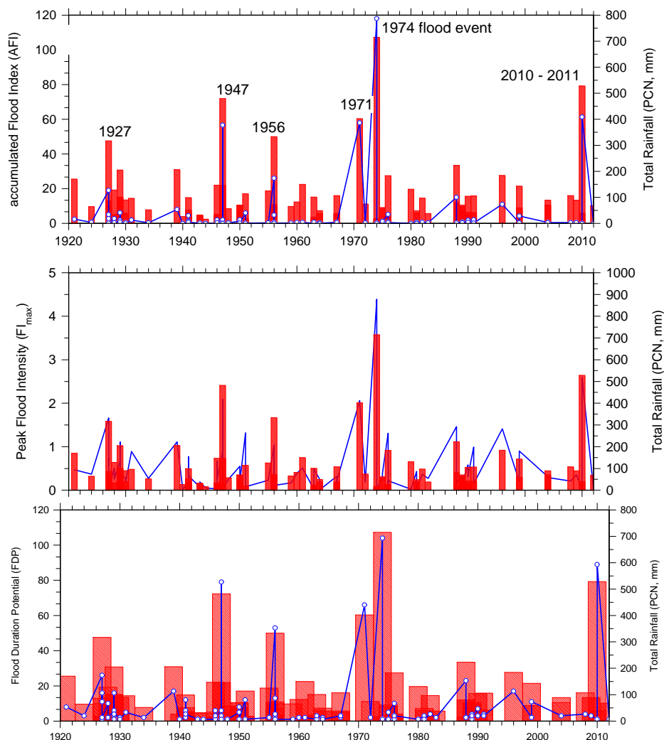
Figure 1. Diagnosis of flood events using Flood Index based on daily effective precipitation. (a) Accumulated flood index (AFI), (b) Peak Flood Intensity ( FI_{\max} ), (c) Flood duration potential (FDP) for
