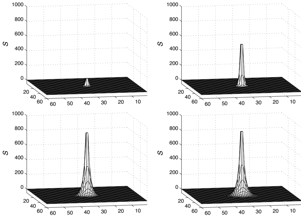
Figure 1: The formation of the stationary soliton. t = 0.425, 0.45, 1.5, 5 . \beta\tau = 10, \lambda\tau = 0.3, \mu\tau = 25, \tau/2 = 0.3 .
