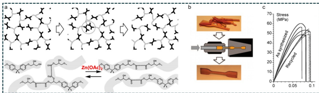
Figure 5. (a) Schematic diagram of the topological rearrangement of the epoxy/carboxylic acid system catalyzed by zinc acetate; (b) Recovery of waste vitrimer by hot pressing; (c) stress-strain curve of the vitrimer before and after recycling. 6 Reproduced or adapted with permission from ref 6. Copyright (2011) The American Association for the Advancement of Science.
