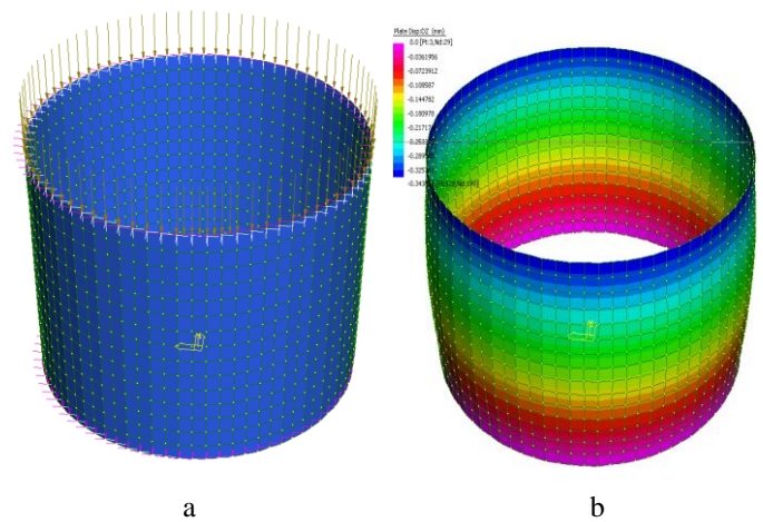
Figure 4. (a) Finite element model (b) deformed mode.
