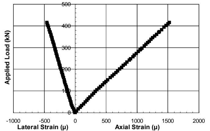
Figure 3. Applied load-strain curve.
