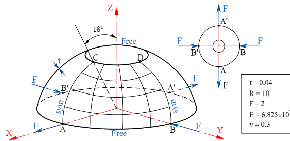
Figure 12: A pinched hemispherical shell with 18° hole: Geometry and material data
