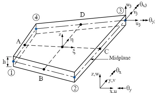
Figure 2: A 4-node quadrilateral plate bending element
