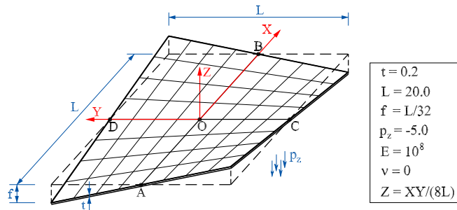
Figure 14: A hyperbolic shell: Geometry and material data
