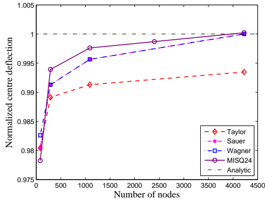
Figure 15: A hyper shell: normalized central deflections with mesh refinement
