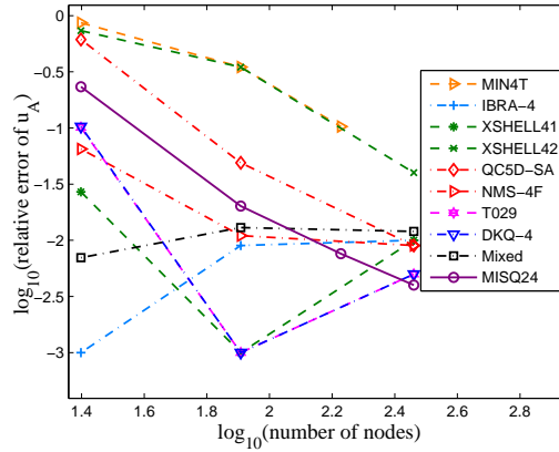
Figure 13: A pinched hemispherical shell with an 18^\circ hole: Convergence behaviour
