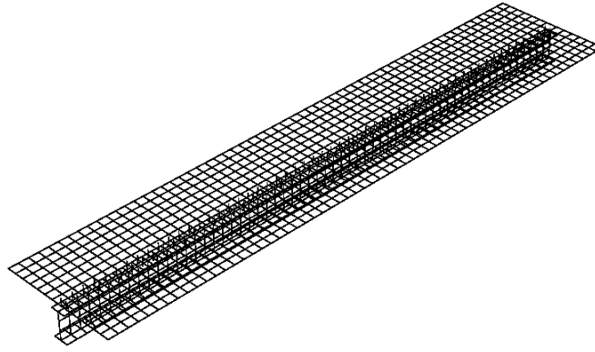
Fig. 1. Typical finite element mesh for the composite beam
