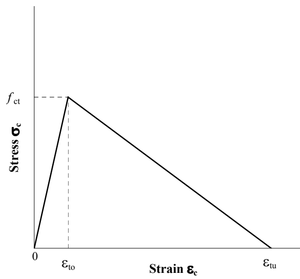
Fig. 4. Stress-strain curve for concrete in tension
