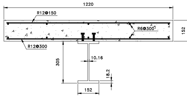
Fig. 5. Cross-section of the composite beam (Chapman and Balakirshnan 1964)
