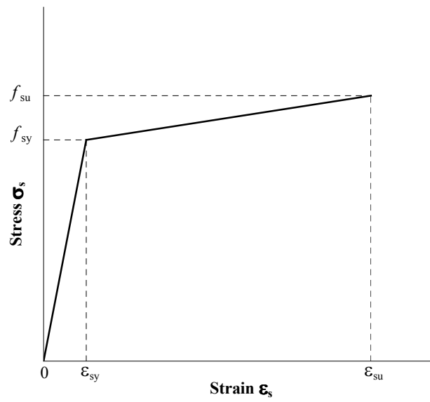
Fig. 2. Stress-strain curve for steel with strain hardening
