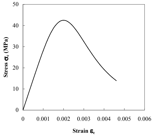
Fig. 3. Stress-strain curve for concrete in compression
