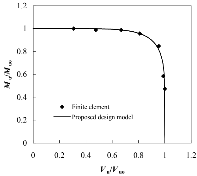
Fig. 8. Moment-shear interaction of composite beams
