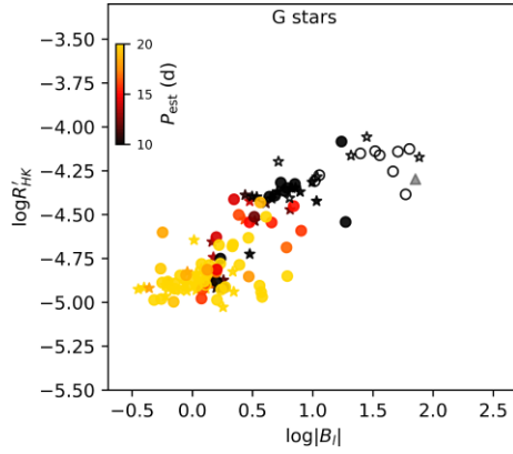
Figure B1. Mean chromospheric activity versus mean longitudinal magnetic field strength for G stars, where colour scales with the estimated rotation period, P_{\text{est}, i=60^\circ} . Marker shapes/styles are the same as in Fig. 1.
