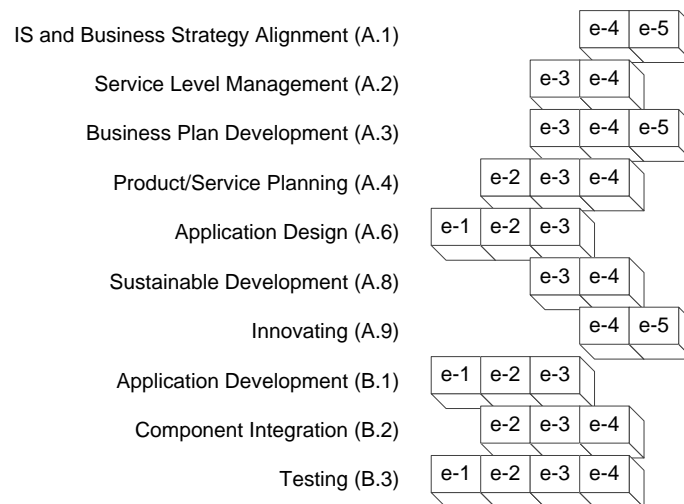
Figure 5: Sample Mapping of Competencies to Levels of Proficiency in e-CF (Own Work)
