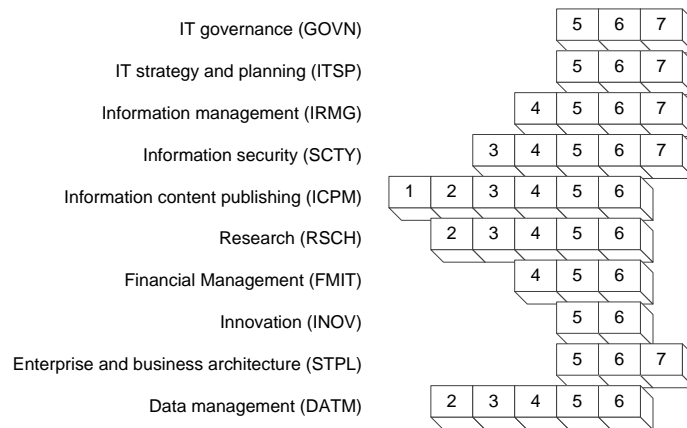
Figure 3: Sample Mapping of Professional Skills to Levels of Responsibility in SFIA (Own Work)
