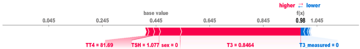
Fig. 6. Local Explanations generated by SHAP force plot, highlighting the most influential features for a random positive case.
