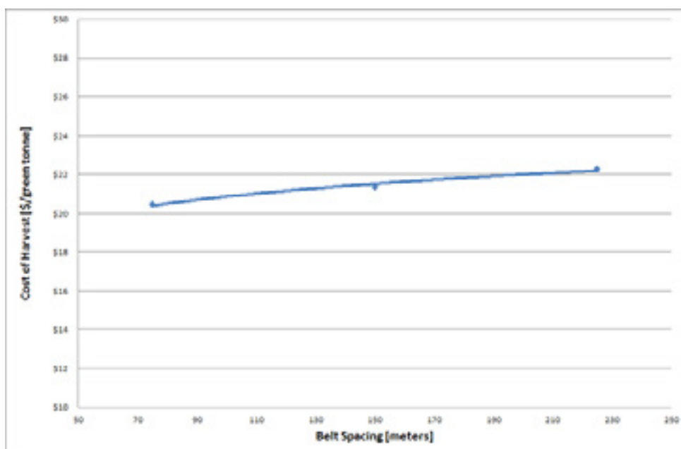
Figure 7.6 Effect of belt spacing on cost of harvest
