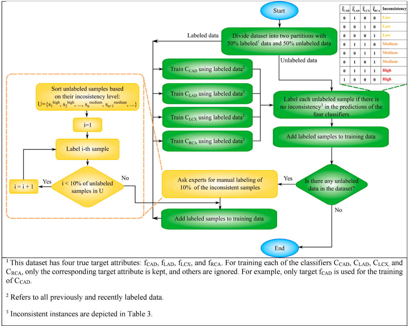
Fig. 8. Flowchart of the proposed method.
