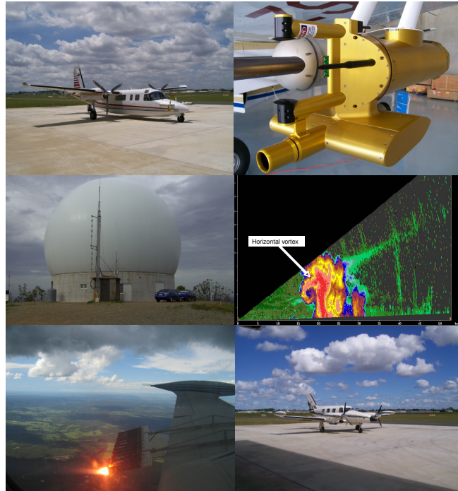
Figure 1: SAWS/WITS Aerocommander 690A research aircraft (upper left), DMT CAPS probe (upper right), BOM/NCAR CP2 dual wavelength polarimetric radar (centre left), vertical section image through a hail storm (centre right), hygroscopic flare in operation below a convective cloud (lower left), WMI/MIPD Cheyenne II randomised seeding aircraft (lower right),
