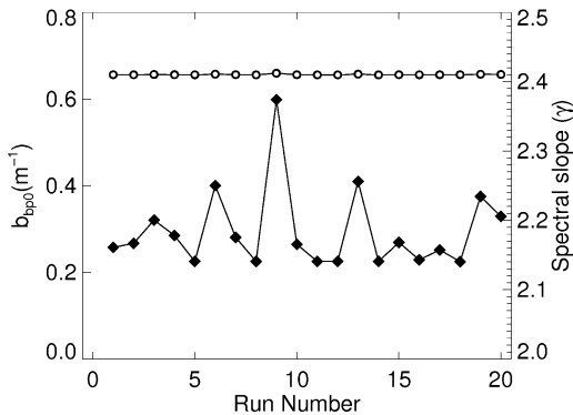
Figure 2 The magnitude of the retrieved bbp0 (closed diamonds) and spectral slope ( \gamma ) (open circles) values for the 20 runs.
