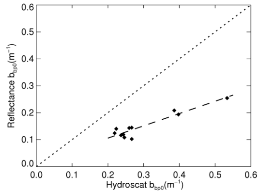
Figure 4 The Hydroscat-6 derived bbp0 vs Reflectance derived bbp0 for the Burdekin Falls Dam stations. The dashed line shows a line of best fit for the data and the dotted line is a 1:1 correspondence line.
