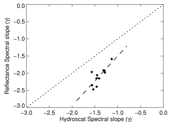
Figure 5 The Hydroscat-6 derived \gamma vs. Reflectance derived \gamma for the Burdekin Falls Dam stations. The dashed line shows a line of best fit for the data and the dotted line is a 1:1 correspondence line.
