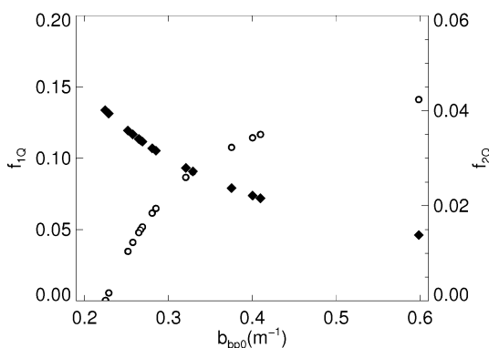
Figure 3 The correlation between the retrieved values of values bbp0 , f_{1Q} (closed diamonds) and f_{2Q} (open circles) for the 20 runs.
