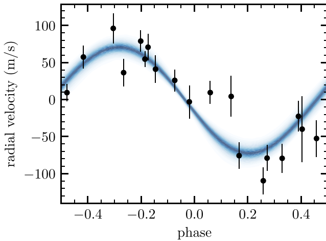
Figure 11. SOPHIE RV (black) with the 99th percentile models from a joint fit with the TESS photometry encapsulated in the blue region. The RV are indicative of a 0.44M_{\text{Jup}} planet, and are in phase with the transits observed by TESS .
