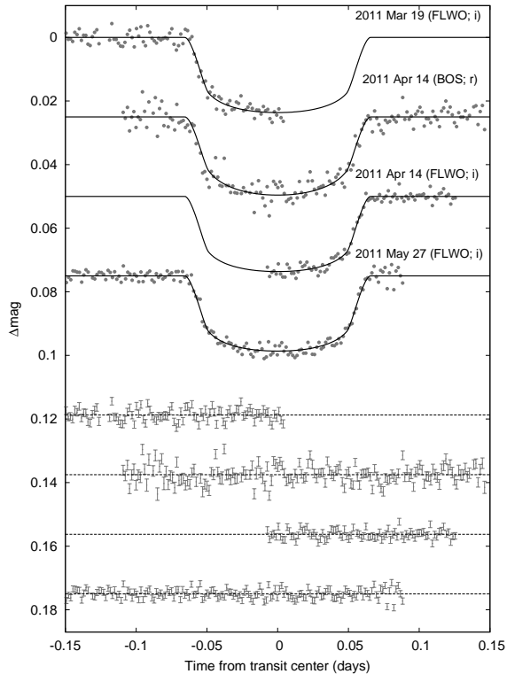
Figure 5. Unbinned transit light curves for HAT-P-44. The light curves have been EPD and TFA processed, as described in § 3.4. The dates of the events, the facilities used to collect the light curves, and the filters used are indicated. Curves after the first are displaced vertically for clarity. Our best fit from the global modeling described in Section 3.4 is shown by the solid lines. Residuals from the fits are displayed at the bottom, in the same order as the top curves. The error bars represent the photon and background shot noise, plus the readout noise.
