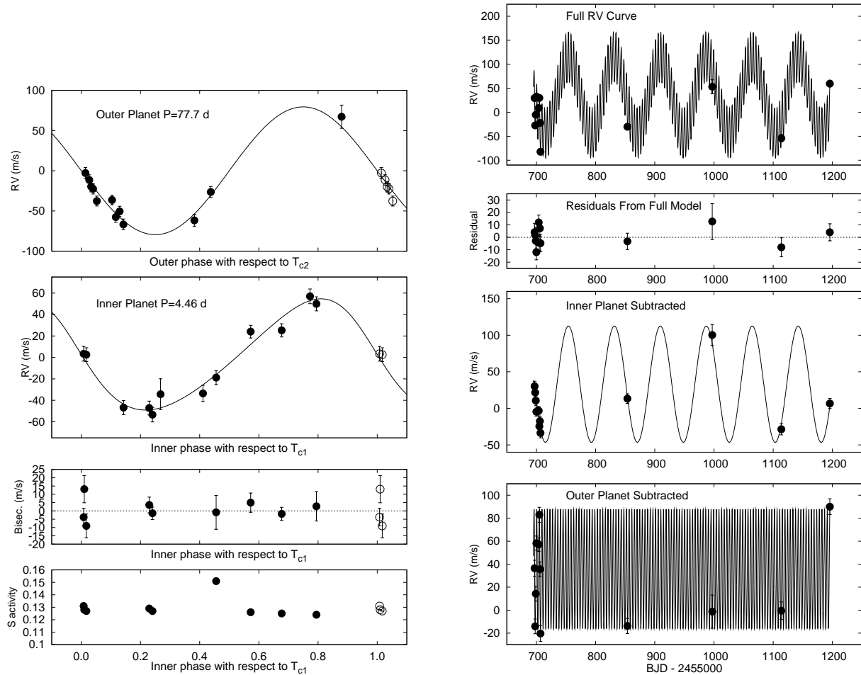
Figure 4. Keck/HIRES observations of HAT-P-46. The panels are as in Figure 2. The parameters used in the best-fit model are given in Table 13.
