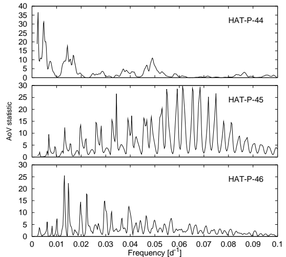
Figure 9. Harmonic AoV periodograms of the RV residuals from the best-fit single planet models for HAT-P-44, HAT-P-45 and HAT-P-46.
