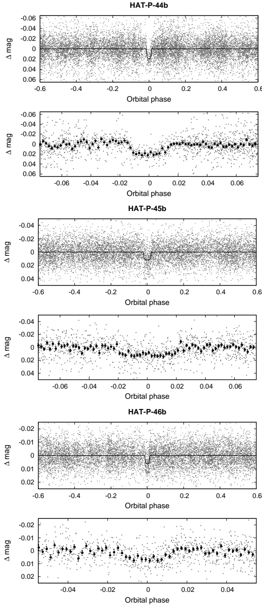
Figure 1. HATNet light curves of HAT-P-44 (top), HAT-P-45 (middle) and HAT-P-46 (bottom). See Table 1 for a summary of the observations. For each planet we show two panels. The top panel shows the unbinned light curve folded with the period resulting from the global fit described in Section 3. The solid line shows the model fit to the light curve (Section 3.4). The bottom panel shows the region zoomed-in on the transit. The dark filled circles show the light curve binned in phase with a bin size of 0.002. These are plotted with 1\sigma uncertainties.
