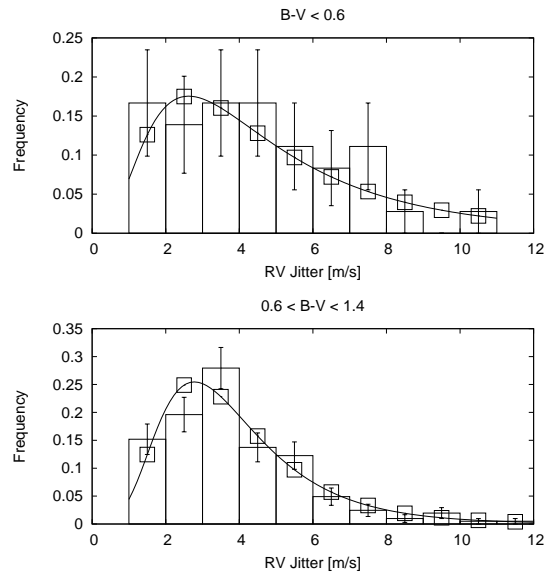
Figure 10. Comparison of the distribution of Keck/HIRES jitter values for low activity main sequence stars taken from Wright (2005) to our model distributions. The histograms show the empirical distributions with Poisson error-bars, the open squares show equation 1 integrated over each bin, and the solid curves are included to show the form of the distribution. The top panel is for stars with B - V < 0.6 , appropriate for HAT-P-45 and HAT-P-46, the bottom panel is for stars with 0.6 < B - V < 1.4 , appropriate for HAT-P-44.
