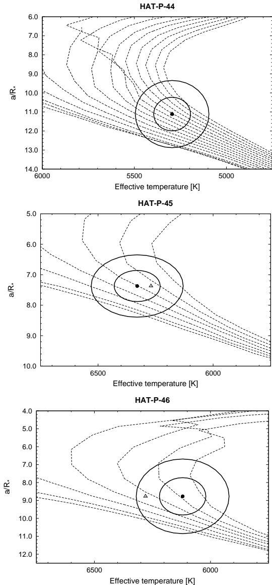
Figure 8. Model isochrones from Yi et al. (2001) for the metallicities of HAT-P-44 (top), HAT-P-45 (center) and HAT-P-46 (bottom). For HAT-P-44 the isochrones are shown for ages of 0.2 Gyr, 0.6 Gyr, and 1.0 Gyr to 13.0 Gyr in steps of 1.0 Gyr (left to right), while for HAT-P-44 and HAT-P-45 the isochrones are shown for ages of 0.2 Gyr, and 0.5 Gyr to 3.0 Gyr in steps of 0.5 Gyr (left to right). The adopted values of T_{\text{eff},*} and a/R_* are shown together with their 1\sigma and 2\sigma confidence ellipsoids. For HAT-P-45 and HAT-P-46 the initial values of T_{\text{eff},*} and a/R_* from the first SME and light curve analyses are represented with a triangle.
