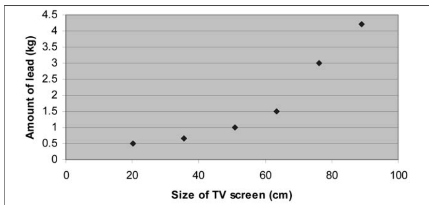
Figure 2. Typical lead content of CRTs.
