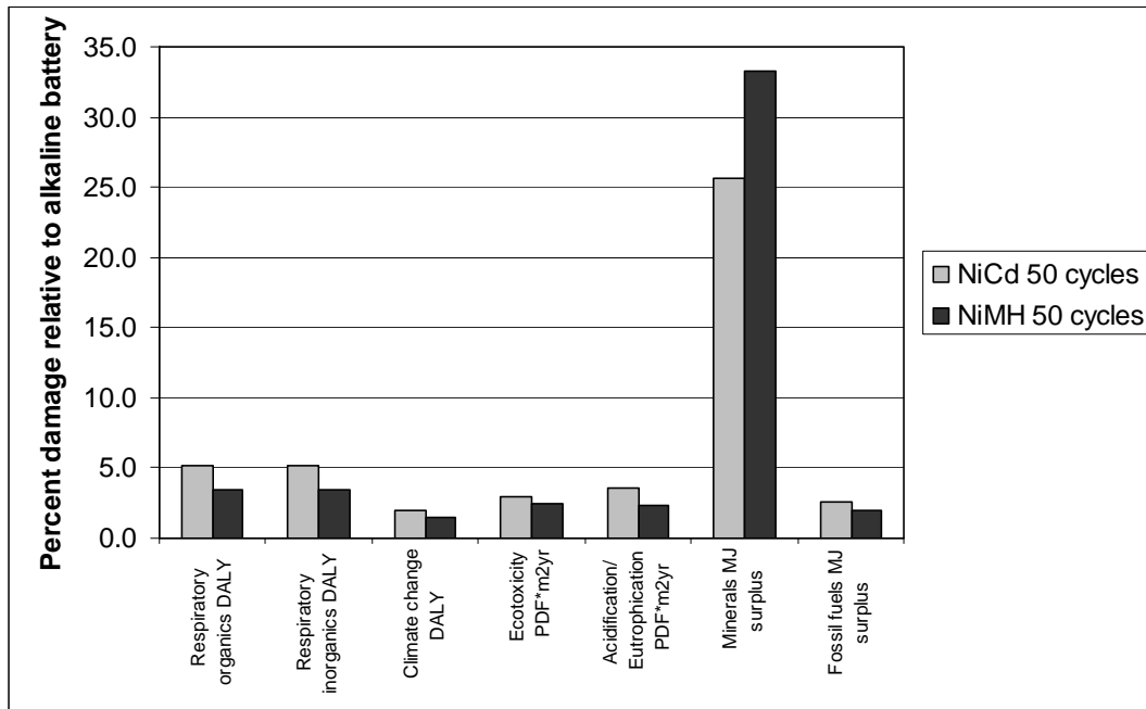
Figure 4. The relative characterization performance of NiCd and NiMH batteries with 50 cycles of discharge and charge to that of Alkaline batteries.
