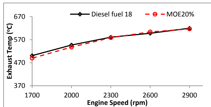
Figure 8. The exhaust gas temperature ( ^{\circ}\text{C} ) at different engine speeds using PD and MOE20%.
