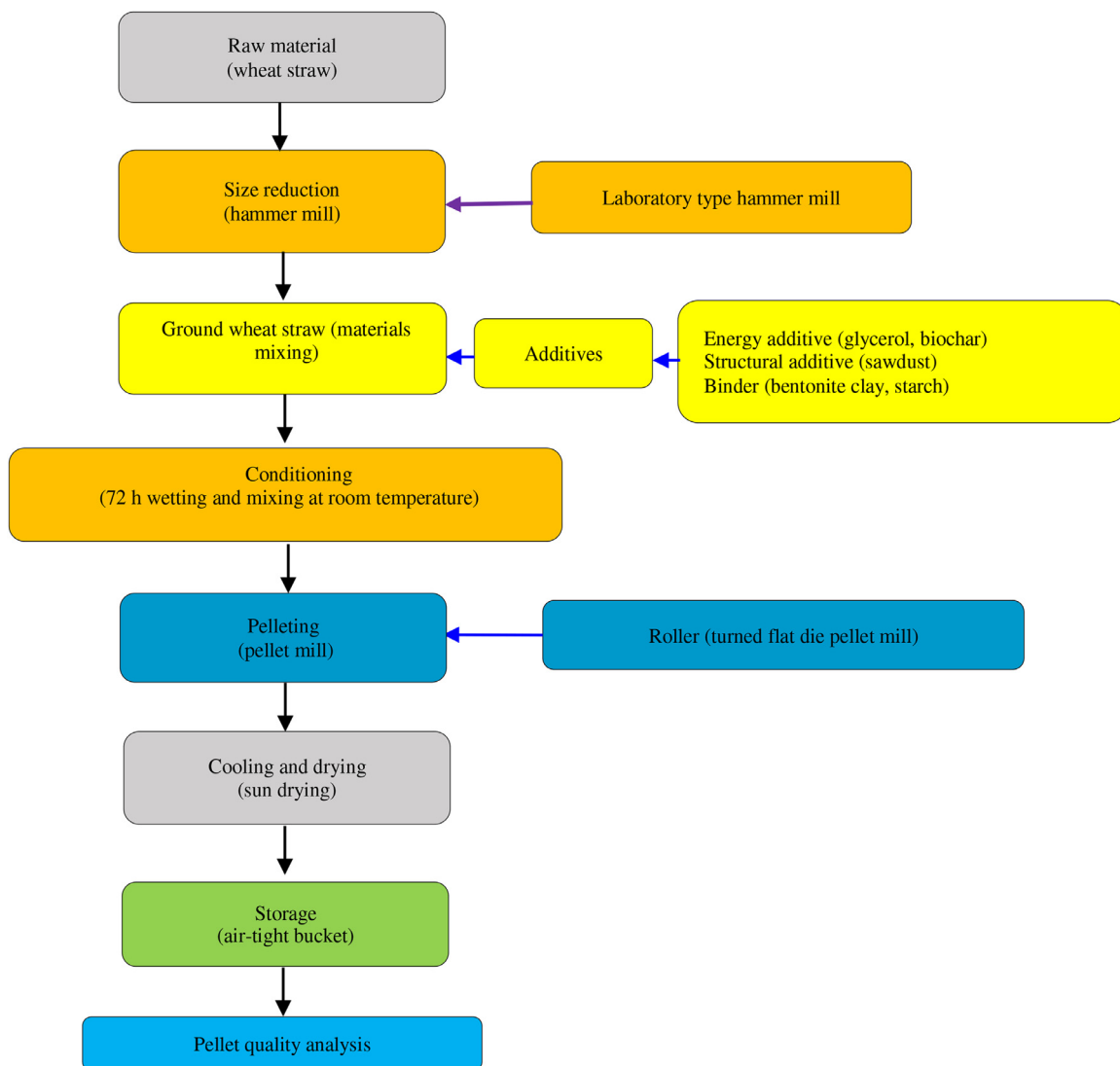
Fig. 1. Flow diagram of pellet production.
