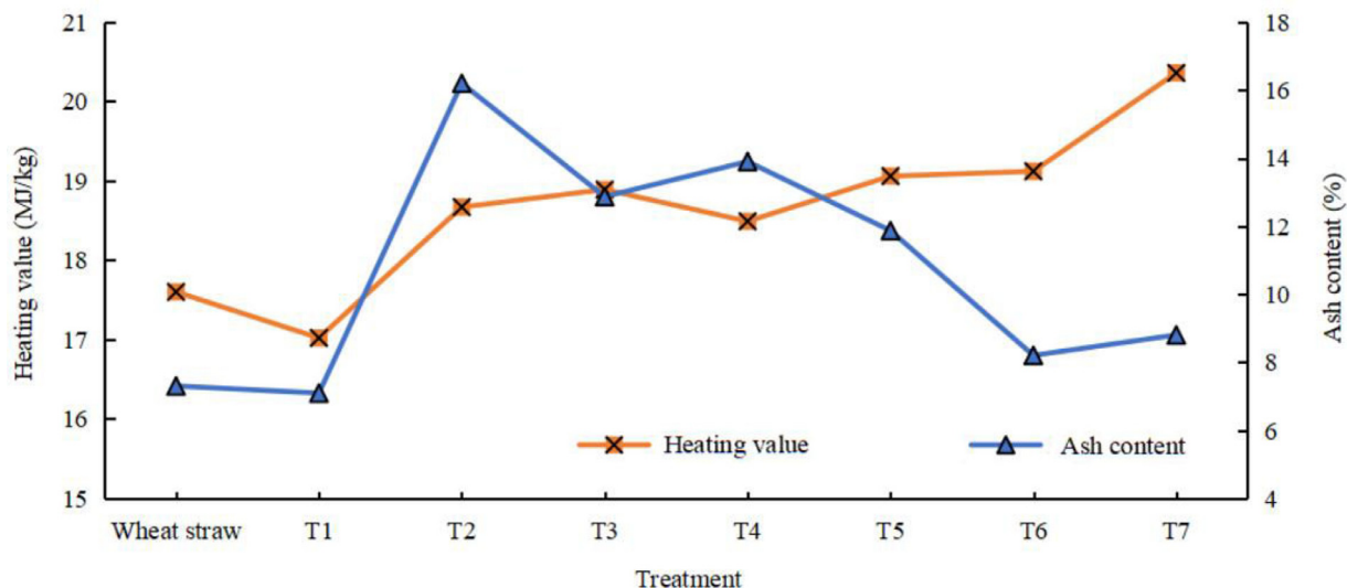
Fig. 5. Combustion properties of pellet.
