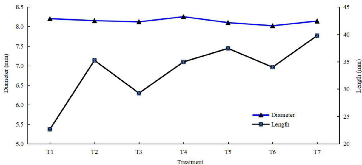
Fig. 4. Length and diameter of pellets.
