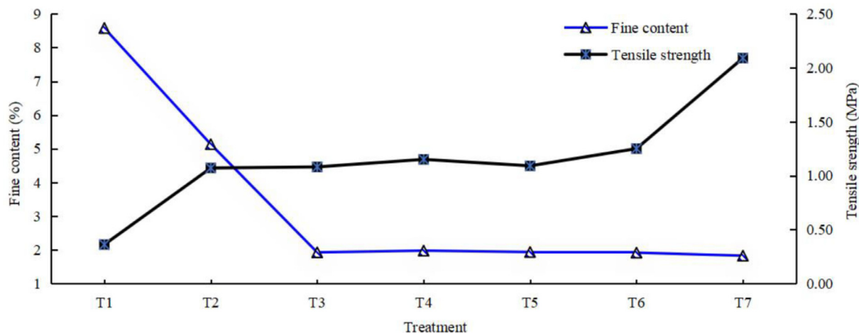
Fig. 8. Fines content and tensile strength.
