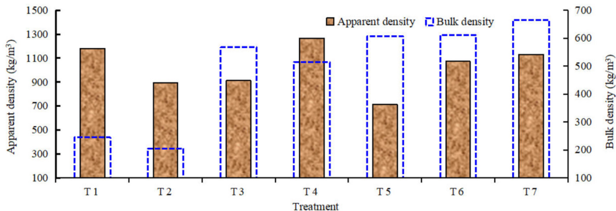
Fig. 6. Bulk density and unit density of pellets.
