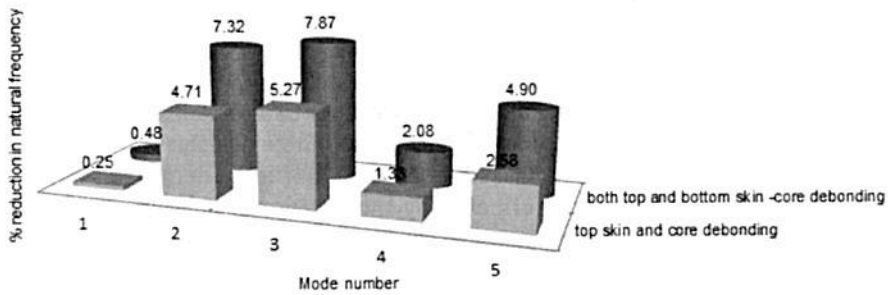
Figure 7. Comparison of percentage natural frequency reduction for single and double layer debonding in 1000 mm C-C-C-C plate for debonding position 3
