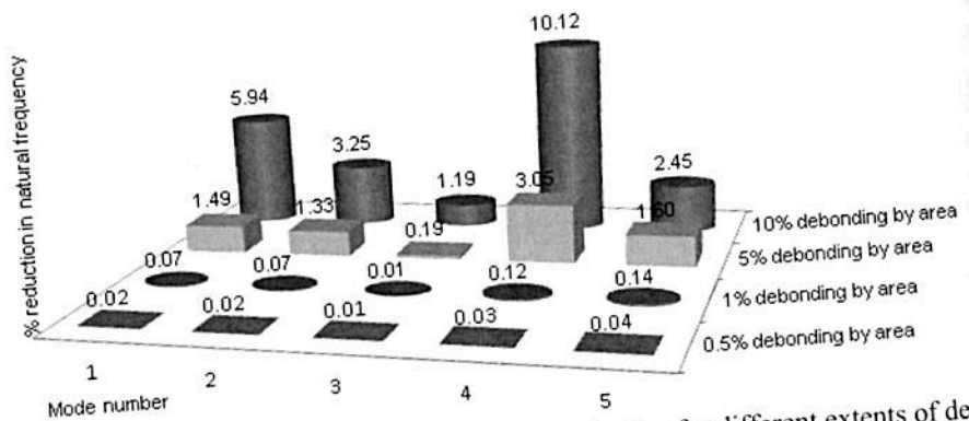
Figure 3. Comparison of percentage natural frequency reduction for different extents of debonding in 800 mm C-C-C-C plate for debonding position 3
