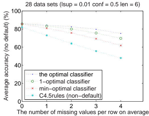
Figure 5: The average accuracies of four classifiers without the default predictions on 28 data sets. Optimal rule classifiers are the most robust, 1-optimal classifiers the second, min-optimal classifiers the third and C4.5rules classifiers the least robust.
