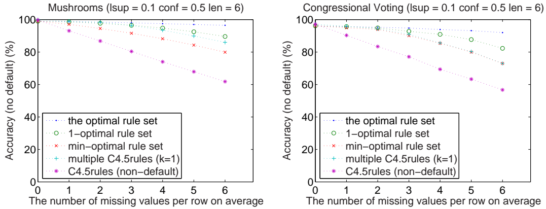
Figure 2: The robustness of different rule sets. Optimal rule sets are the more robust, 1-optimal rule sets the second, min-optimal rule set the third, and rule sets from C4.5rules the least robust. Rule sets from multiple C4.5rules are more robust than rule sets from single C4.5rules but less robust than 1-optimal rule sets.
