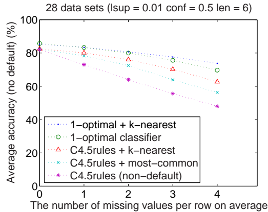
Figure 6: The comparison of 1-optimal classifier with two missing value imputation methods on 28 data sets. The 1-optimal classifier is more accurate than C4.5rules plus two imputation methods respectively in the presence of missing values.
