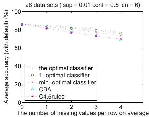
Figure 4: The average accuracies of five classifiers with the default predictions on 28 data sets. Optimal, 1-optimal and min-optimal classifiers (top three lines) are more robust than CBA classifiers and C4.5rules classifiers.
