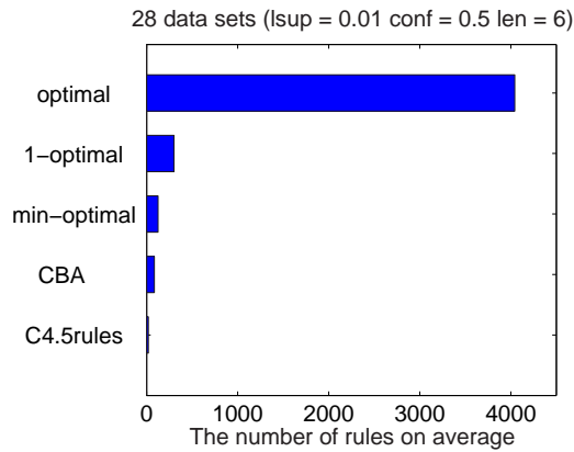
Figure 3: The average sizes of different classifiers on 28 data sets. An optimal classifier is large whereas a C4.5rules classifier is very small. A CBA classifier is close to a min-optimal classifier, and both are smaller than a 1-optimal classifier.
