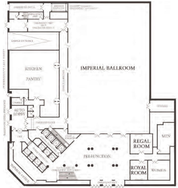
B-2 LEVEL
