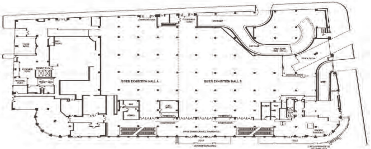
LEVEL ONE
