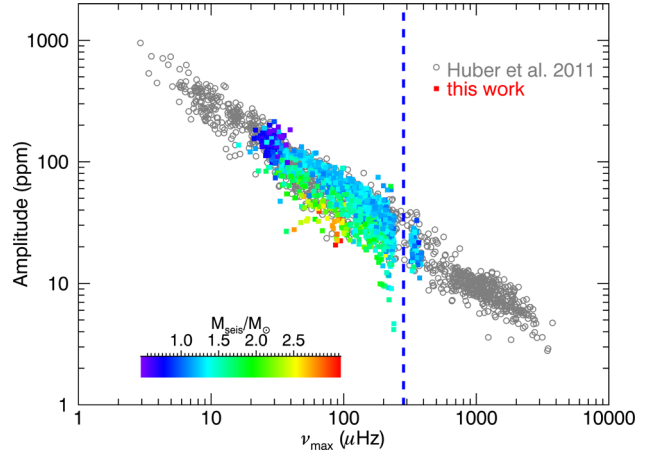
Figure 4. Oscillation amplitude at \nu_{\max} against \nu_{\max} for the whole sample (colour coded by the seismic mass). Targets from Huber et al. (2011) are plotted as grey circles. The blue-dashed line denotes the Nyquist frequency (283.22 \mu\text{Hz} ). Targets oscillating near the Nyquist frequency have underestimated amplitudes (see text).
