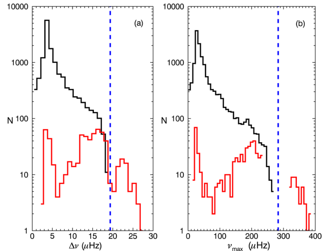
Figure 7. Histograms of \Delta\nu and \nu_{\max} . Red curve represents our sample while black curve indicates Huber et al. (2011) and Stello et al. (2013) samples. The blue-dashed lines mark the Nyquist frequency in panel (b) and its corresponding \Delta\nu calculated from scaling relation in panel (a). The short-cadence sample by Huber et al. (2011) is not shown here.
