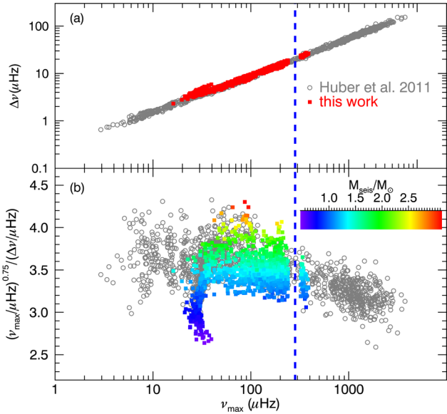
Figure 3. (a): \Delta\nu versus \nu_{\max} for the entire sample (red squares) and those from Huber et al. (2011, grey circles). (b): \nu_{\max}^{0.75}/\Delta\nu versus \nu_{\max} . The blue-dashed line denotes the Nyquist frequency (283.22 \mu\text{Hz} ). Asteroseismic masses are colour coded, which were derived by combining \nu_{\max} , \Delta\nu and KIC effective temperature. We can see clearly the diversity of masses dominates the scatter in the vertical direction. Note that we excluded the stars with measured \nu_{\max} in the range of 240 and 320 \mu\text{Hz} (see text).
