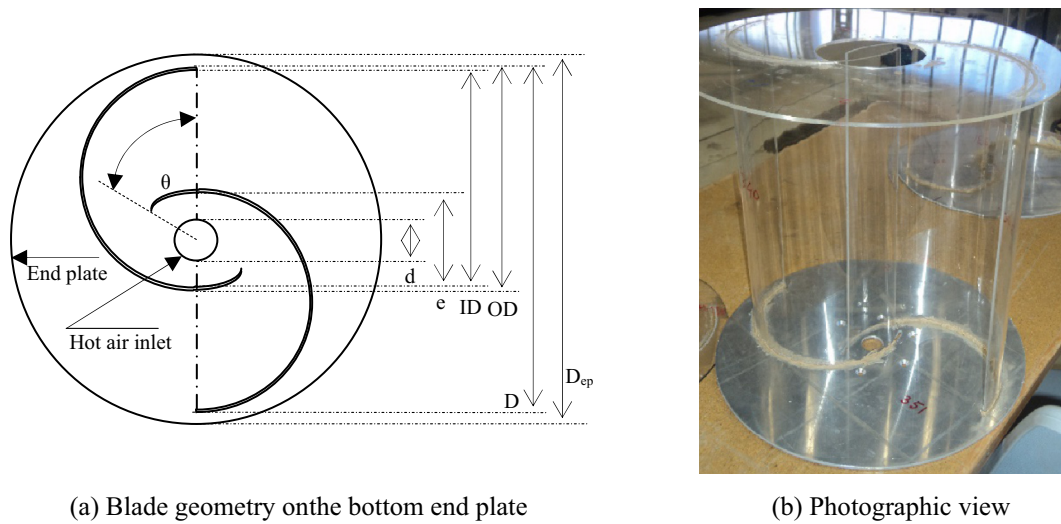
Figure 1 The swirling Savonius rotor.
