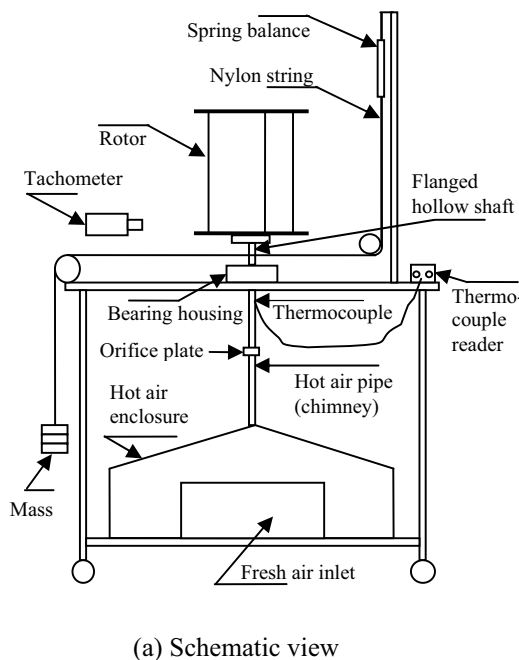
Figure 3 Experimental set-up.
