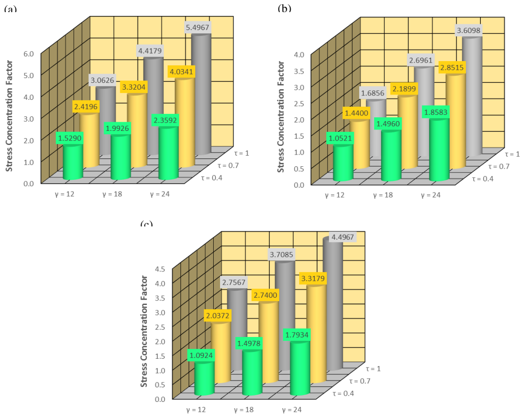
Fig. 8. Effect of the \gamma on the SCFs under the 1 st IPB loading condition ( \theta = 45^\circ , \beta = 0.4 ): (a) Crown position, (b) Toe position, (c) Heel position
