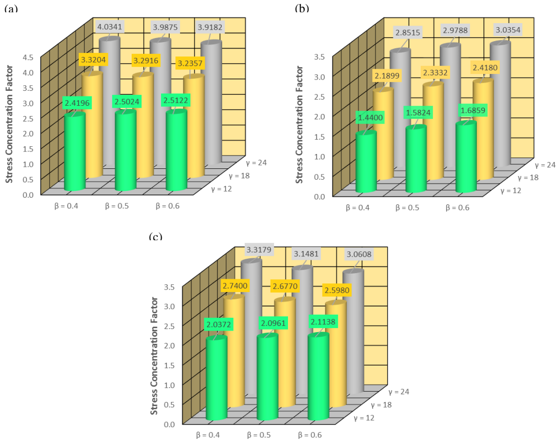
Fig. 7. Effect of the \beta on the SCFs under the 1 st IPB loading condition ( \theta = 45^\circ , \tau = 0.7 ): (a) Crown position, (b) Toe position, (c) Heel position
