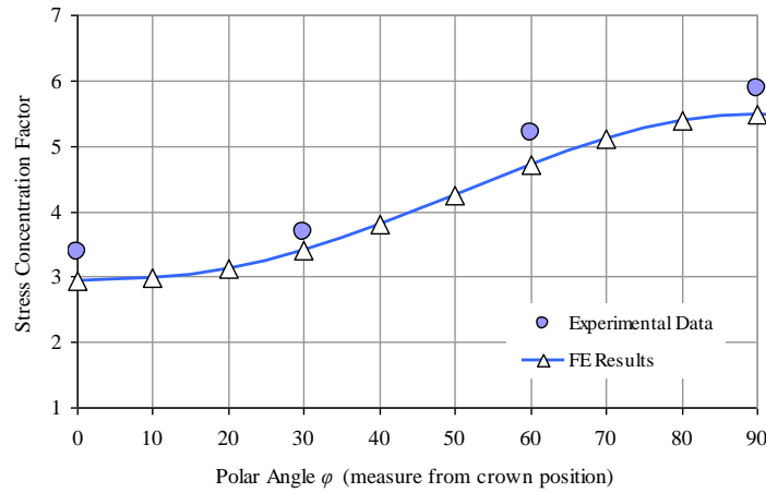
Fig. 5. Distribution of chord-side SCFs along the central brace/chord intersection of uniplanar KT-joint: Comparison of the experimental data and FE results
