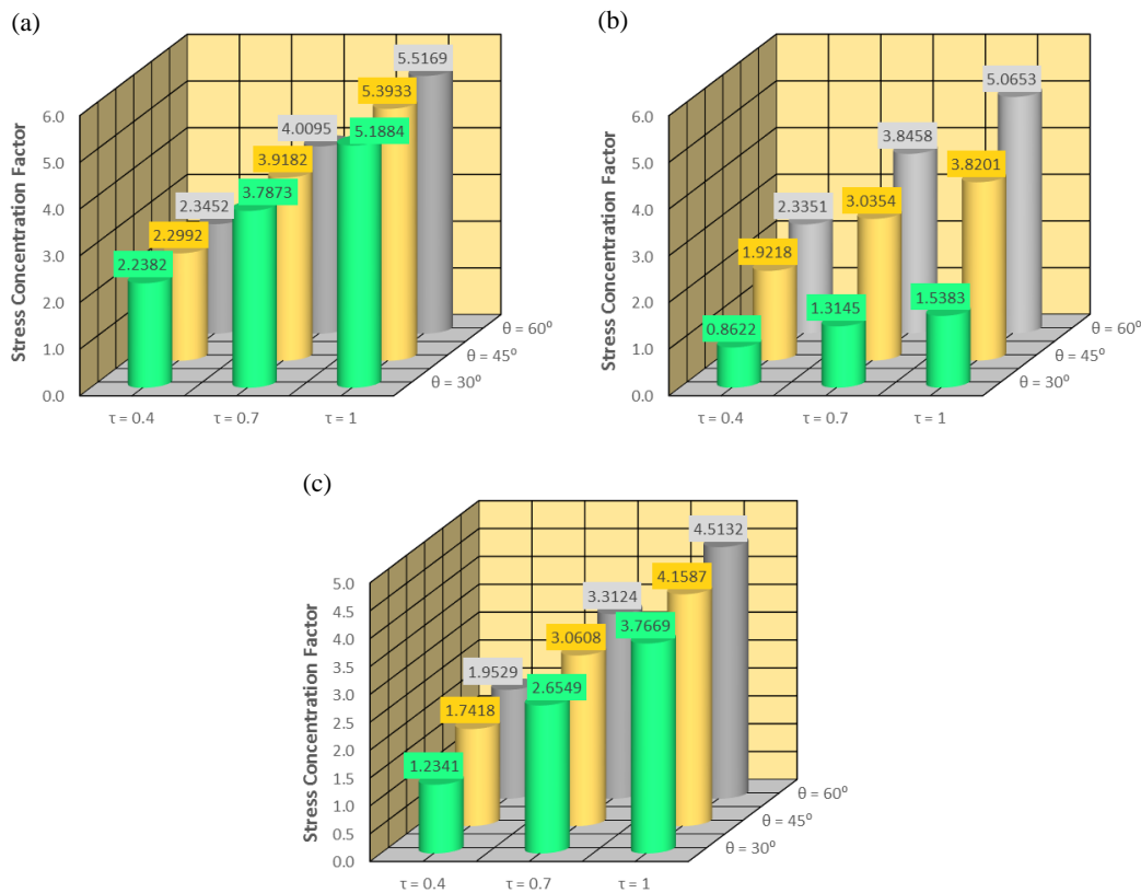
Fig. 6. Effect of the \tau on the SCFs under the 1 st IPB loading condition ( \beta = 0.6 , \gamma = 24 ): (a) Crown position, (b) Toe position, (c) Heel position
