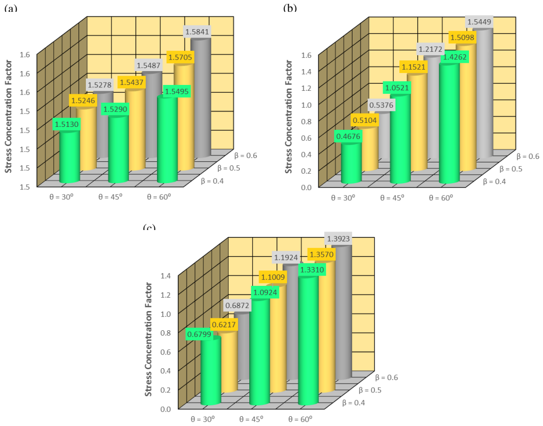
Fig. 9. Effect of the \theta on the SCFs under the 1 st IPB loading condition ( \tau = 0.4, \gamma = 12 ): (a) Crown position, (b) Toe position, (c) Heel position
