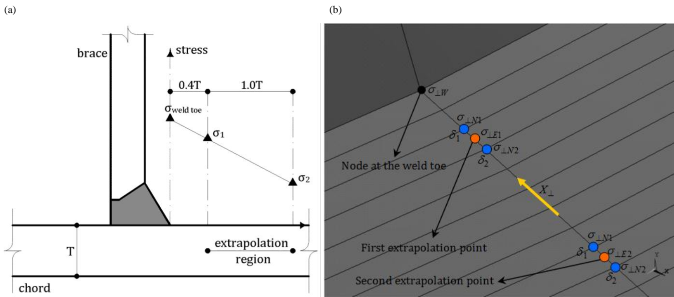
Fig. 4. (a) Extrapolation procedure recommended by IIW-XV-E [51], (b) Required interpolations and extrapolations to extract SCFs based on the stresses perpendicular to the weld toe
