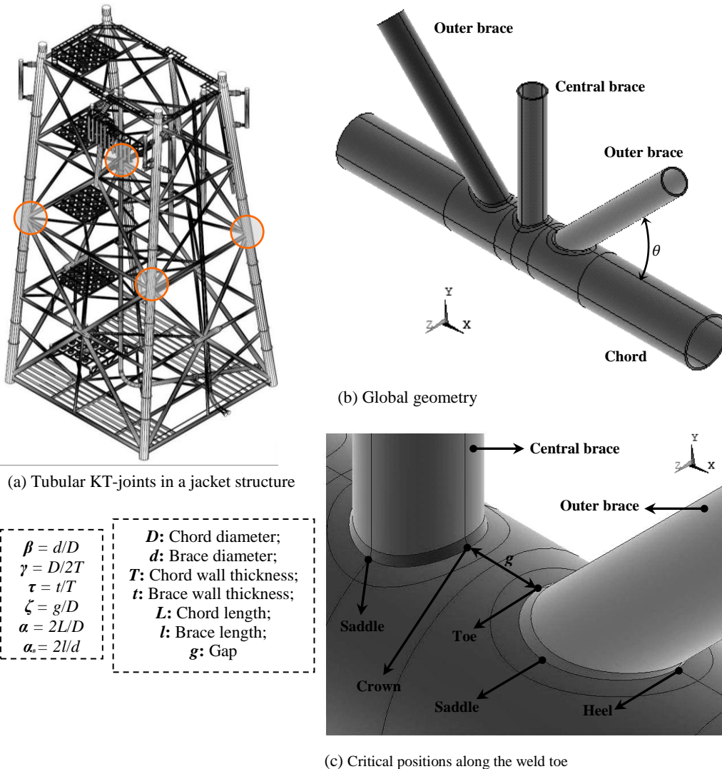
Fig. 1. Geometrical notation for a simple uniplanar KT-joint
