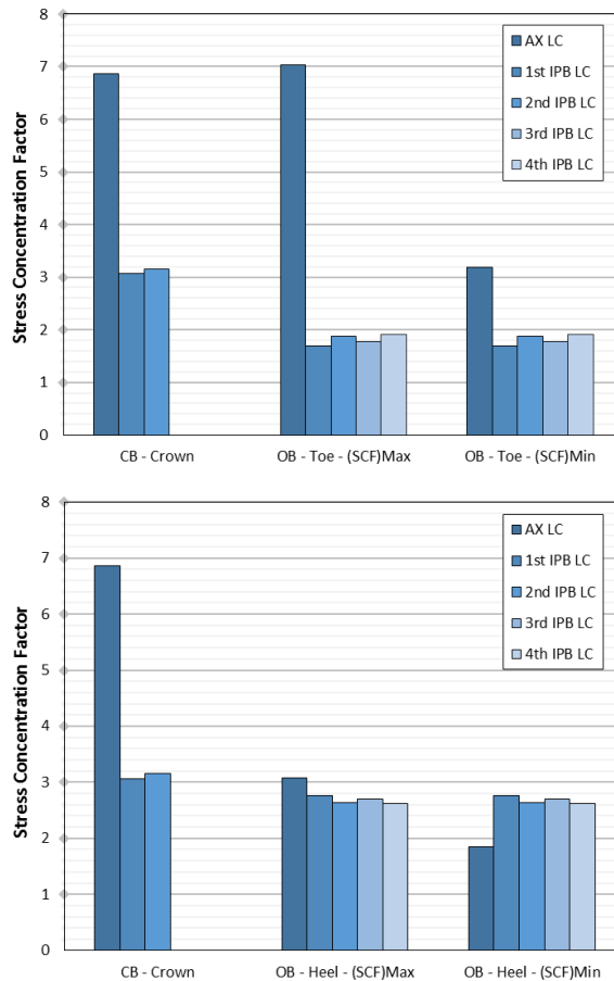
Fig. 10. Comparison of chord-side SCFs under axial and IPB loading conditions ( \theta = 45^\circ, \beta = 0.4, \tau = 1.0, \gamma = 12 )
