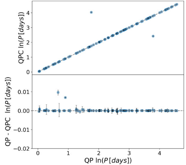
Figure 7. This figure compares the QP and QPC solution for \ln(\text{Period}) . Figure description is same as Fig. 3.
