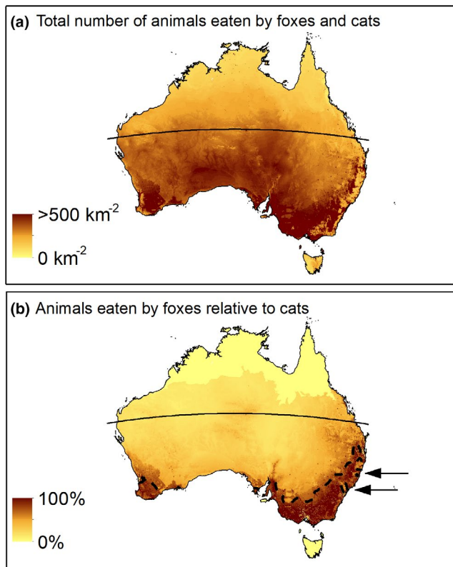
FIGURE 4 (a) The estimated total number of animals (including only reptiles, birds and mammals) eaten by foxes and cats combined each year throughout Australia, and (b) the proportion of this total that is attributable to fox predation; dashed line indicates where the number of animals eaten by foxes versus cats is relatively equal (50%). Solid black line indicates the Tropic of Capricorn
