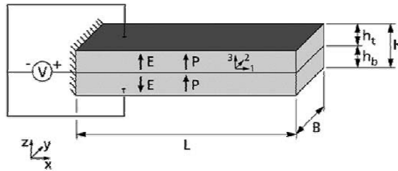
Figure 14: Two-layer parallel bimorph cantilever beam.
