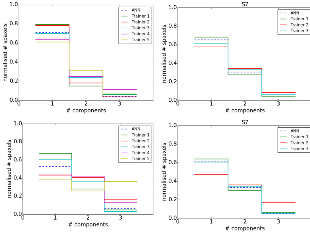
Figure 11. Top: a representation of how many 1-, 2- or 3-component classifications made by each trainer (—) and ANN (---) for the SAMI (left) and S7 (right) on the first training set of galaxies. Bottom: a representation of how many 1-, 2- or 3-component classifications made by each trainer (—) and ANN (---) for the second testing set of galaxies. In both testing sets the ANN predicts similar numbers of 1-, 2- or 3-components for the different surveys.
