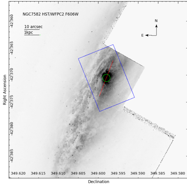
Figure 16. HST image of NGC 7582. Blue box indicates the S7 FoV and the red line shows the major axis of the galaxy we have used in our analysis of the WiFeS data. The green circle indicates the centre of the galaxy.
