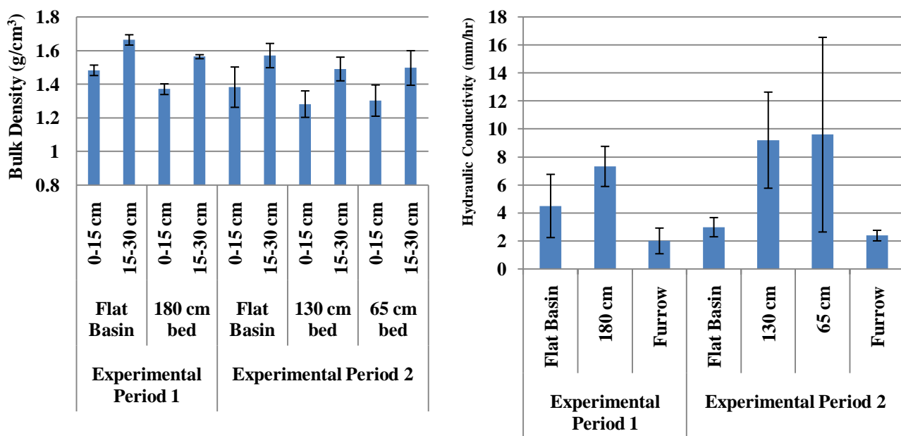
Figure 1: Effect of bed configuration and renovation on hydraulic conductivity and bulk density of a clay loam soil (Mardan, Pakistan). Bars show +/- standard deviation.
