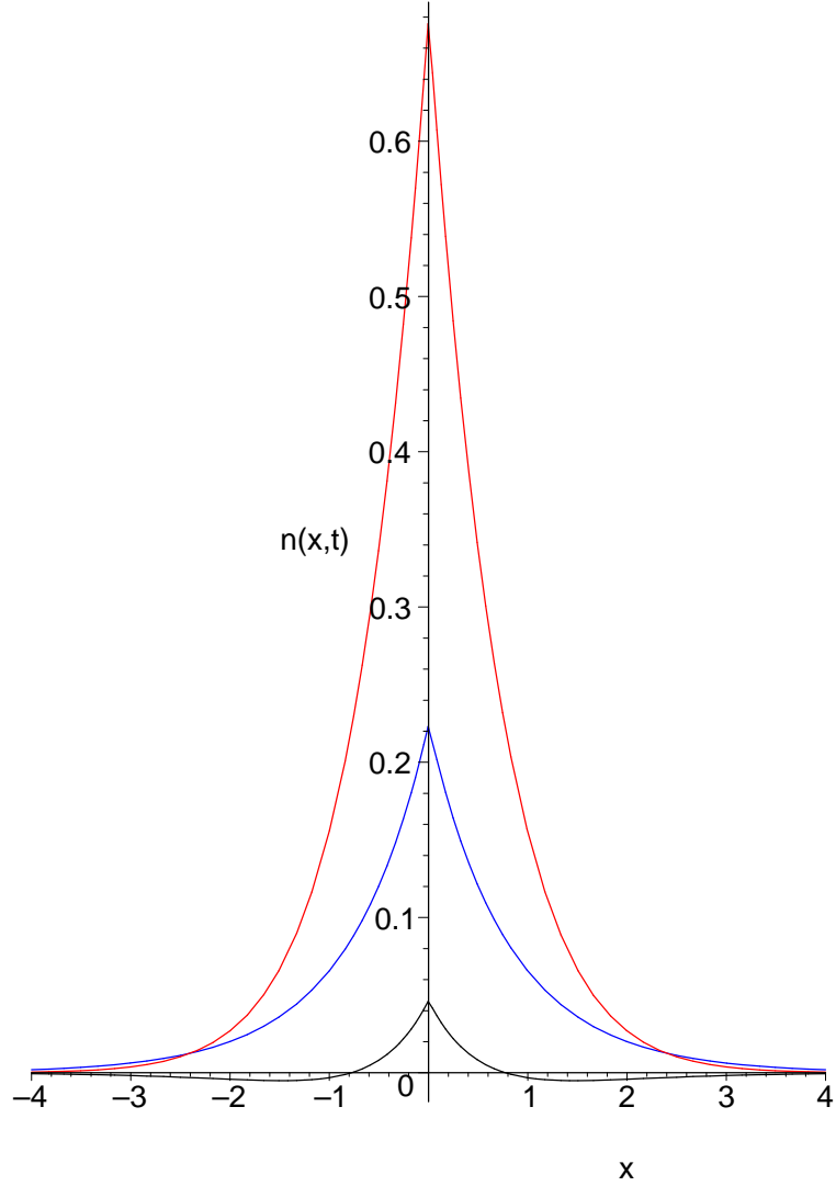
FIG. 1: (Color online) The infinite solution for Model I at the dimensionless times t=0.1 (red), 1.0 (blue), and 5.0 (black) with K = -1 , D = 1 , and \alpha = 1/2 . The peak height decreases with increasing time.
