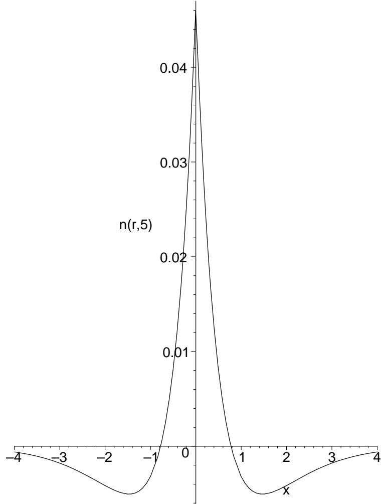
FIG. 4: (Color online) The infinite solution for Model I at the dimensionless time t=5.0 with K = -1 , D = 1 , and \alpha = 1/2 .
