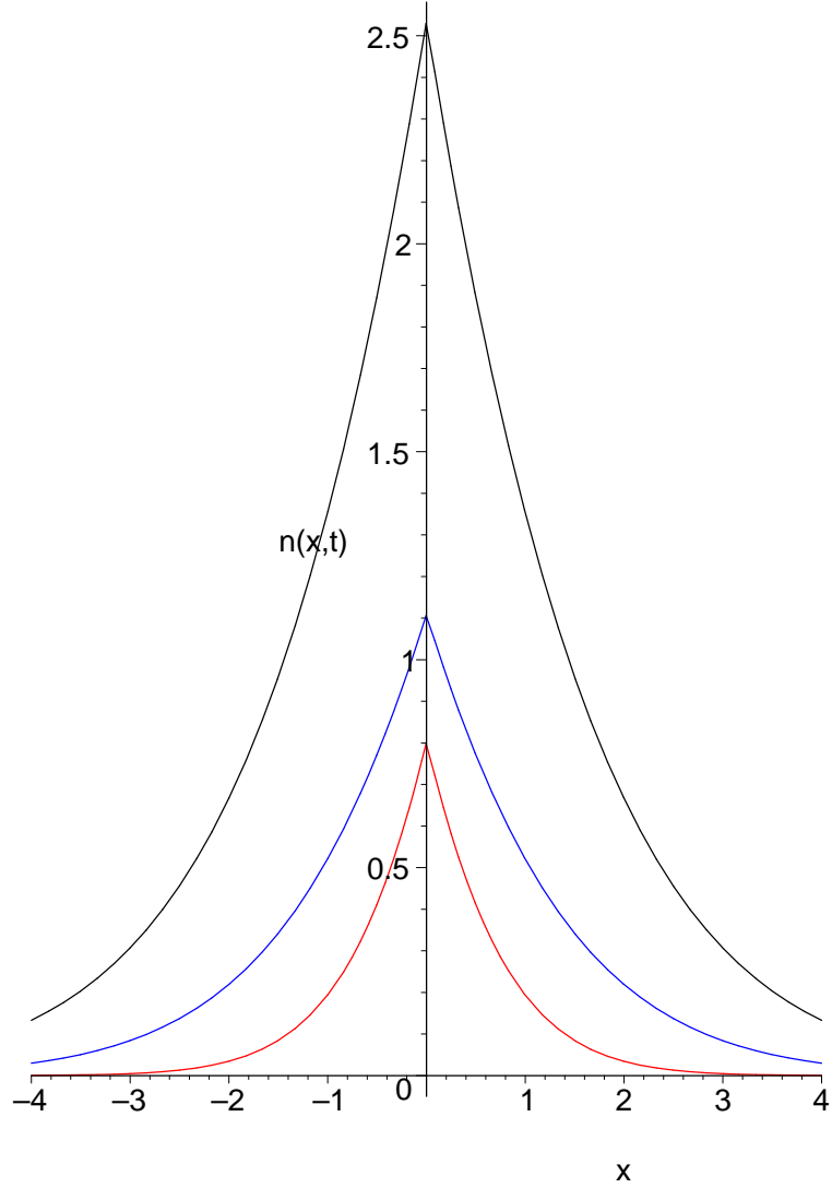
FIG. 9: (Color online) The infinite solution for Model III at the dimensionless times t=0.1 (red), 1.0 (blue), and 2.0 (black) with K = 1 , D = 1 , and \alpha = 1/2 . The peak height increases with increasing time.
