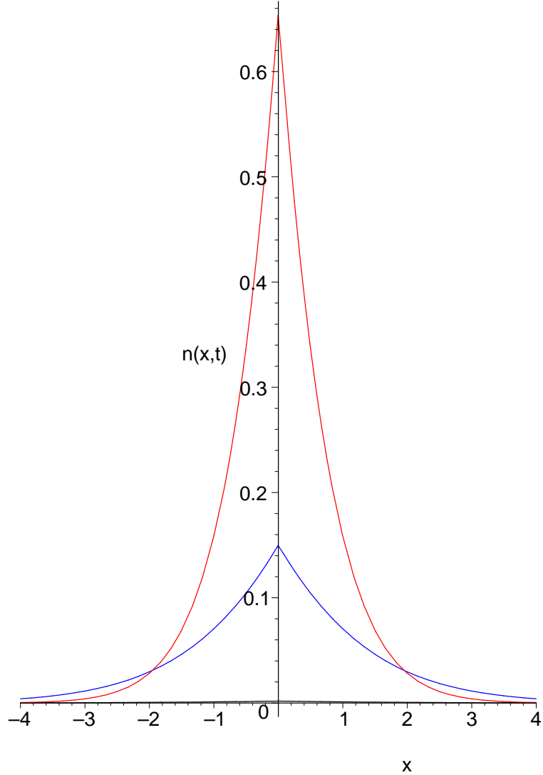
FIG. 3: (Color online) The infinite solution for Model III at the dimensionless times t=0.1 (red), 1.0 (blue), and 5.0 (black) with K = -1 , D = 1 , and \alpha = 1/2 . The peak height decreases with increasing time. The profile at t = 5.0 lies along the x axis.
