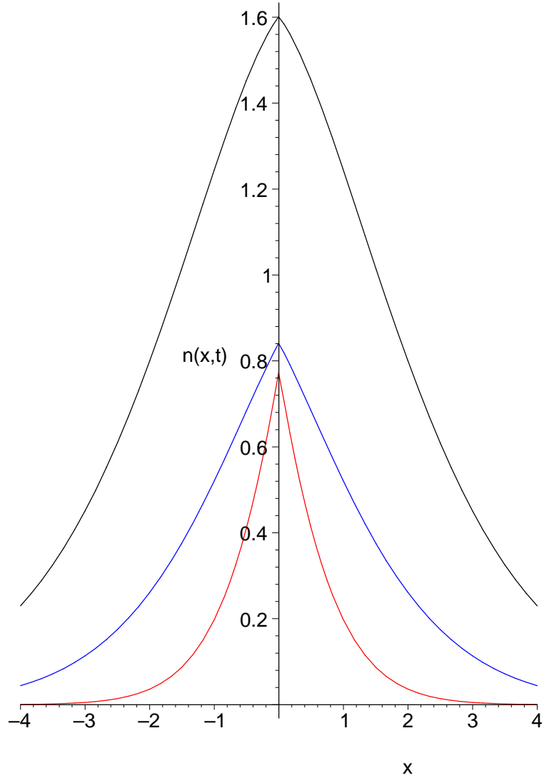
FIG. 7: (Color online) The infinite solution for Model I at the dimensionless times t=0.1 (red), 1.0 (blue), and 5.0 (black) with K = 1 , D = 1 , and \alpha = 1/2 . The peak height increases with increasing time.
