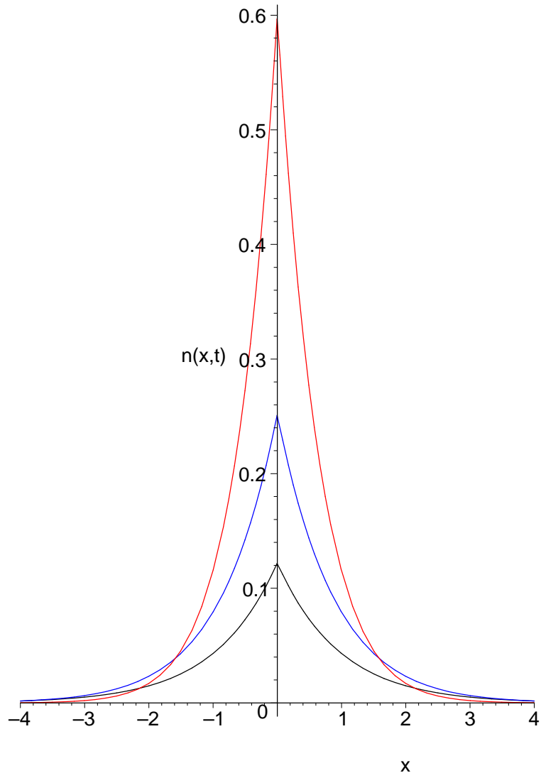
FIG. 2: (Color online) The infinite solution for Model II at the dimensionless times t=0.1 (red), 1.0 (blue), and 5.0 (black) with K = -1 , D = 1 , and \alpha = 1/2 . The peak height decreases with increasing time.
