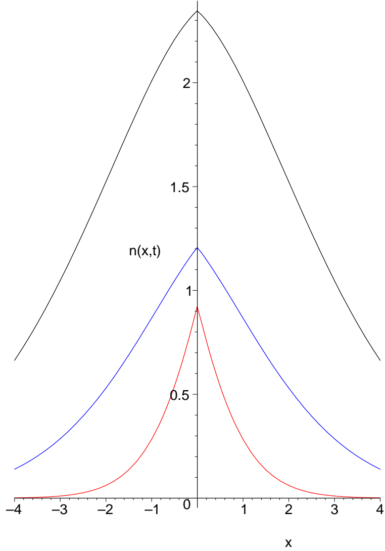
FIG. 8: (Color online) The infinite solution for Model II at the dimensionless times t=0.1 (red), 1.0 (blue), and 2.0 (black) with K = 1 , D = 1 , and \alpha = 1/2 . The peak height increases with increasing time.
