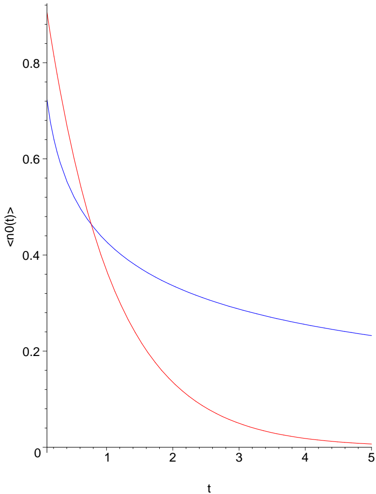
FIG. 5: (Color online) The zeroth order moments of the infinite solution for Models I and III (red), and Model II (blue) with K = -1 , D = 1 , and \alpha = 1/2 . The result for Model II is the upper curve at t = 5 .
