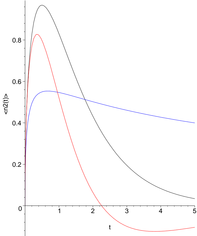
FIG. 6: (Color online) The second order moments of the infinite solution for Models I (red), II (blue), and III (black) with K = -1 , D = 1 , and \alpha = 1/2 . At t = 5 the result for Model II is the upper curve and the result for Model I is the lower curve.
