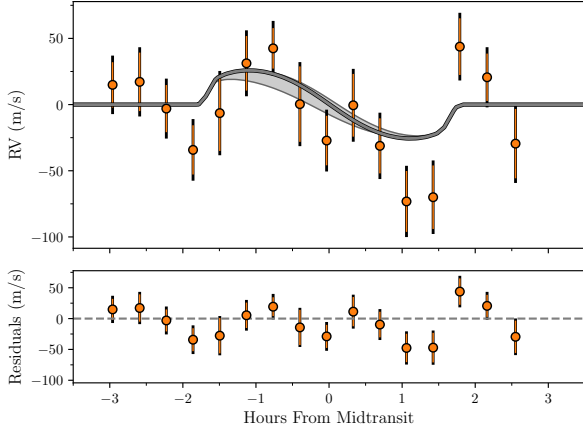
Fig. 8. Rossiter-McLaughlin effect in TOI-2025. Our in-transit observations of TOI-2025 with FIES+. Top: Keplerian orbit and quadratic trend has been subtracted from the RVs to better show the RM effect, with the grey line being the best-fitting model. The shaded area denotes the confidence interval in the projected obliquity, \lambda = 9^{+33}_{-31}^\circ . Bottom: here we have further subtracted this best-fitting model from the RVs.
