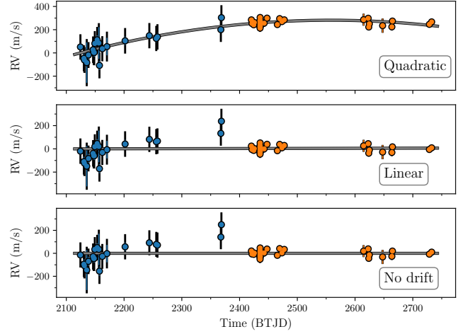
Fig. 9. Long-term trend in TOI-2025. The symbols are the same as in Fig. 5, but here the RVs are plotted against time, and we have subtracted the planetary signal. Top: fit where we allow for a quadratic trend. Middle: fit where we only allow for a linear trend. Bottom: here we do not include any long-term drift.
