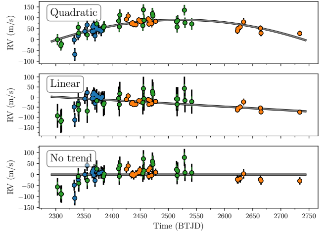
Fig. 10. Long-term trend in TOI-2158. The symbols are the same as in Fig. 5, but here the RVs are plotted against time, and we have subtracted the planetary signal. Top: fit where we allow for a quadratic trend. Middle: here we only allow for a linear trend. Bottom: here we do not include any long-term drift.
