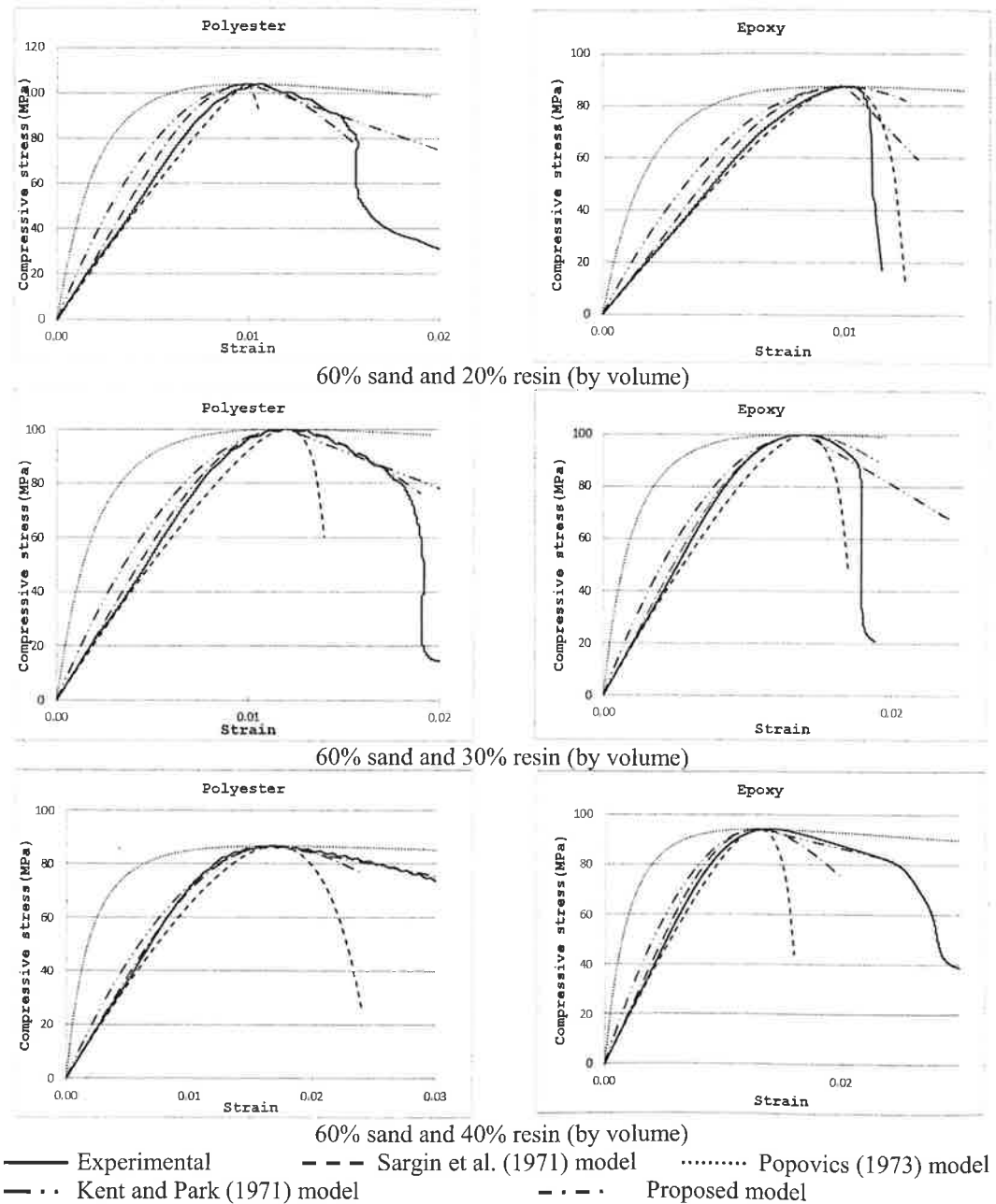
Figure 2. Experimental and predicted stress-strain relationships
