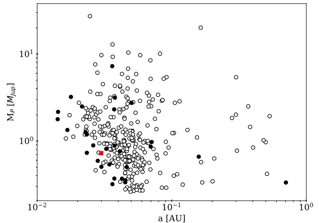
Figure 7. Planet mass as a function of semi-major axis for all known giant ( M_P > 0.25M_J ) planets with measured masses and radii. We differentiate host star masses by plotting the data for stars with < 0.8M_\odot (as filled black circles), for stars with > 0.8M_\odot (as unfilled black circles), and for HAT-P-68b (red square with errorbars). Data from NASA Exoplanet Archive as of 2020 September 24.
