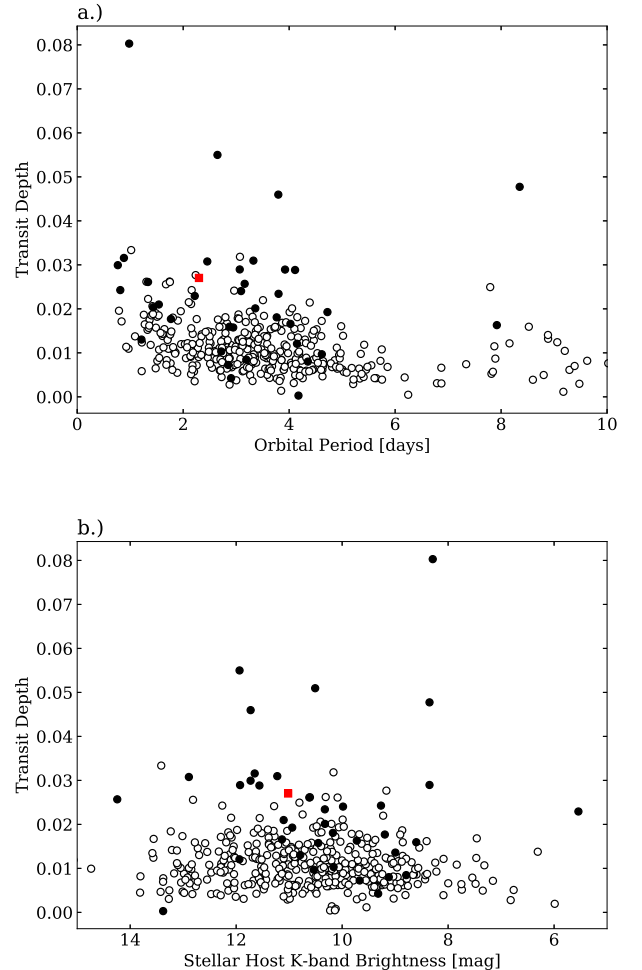
Figure 8. Transit depth as a function of (a.) orbital period for hot Jupiters and (b.) host K -band magnitude. The depth was calculated from the planetary radius R_P and stellar radius R_* . We differentiate host star masses by plotting the data for stars with < 0.8M_{\odot} (as filled black circles), for stars with > 0.8M_{\odot} (as unfilled black circles), and for HAT-P-68b (red square with errorbars). Data from NASA Exoplanet Archive as of 2020 September 24.
