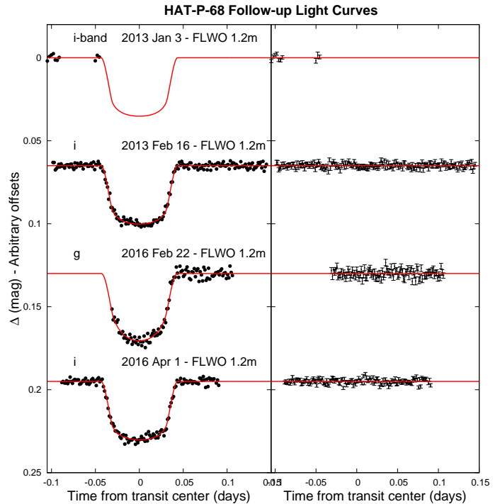
Figure 4. Unbinned follow-up transit light curves obtained with KeplerCam on the FLWO 1.2 m, plotted with the best-fit transit model as a solid red line. The dates of observation and photometric filters used are indicated. The residuals are shown on the right-hand side in the same order as the light curves.
