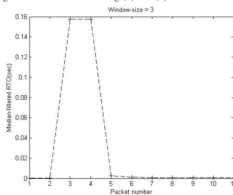
Fig. 8. Smoothed RTO using (2) and (3)
