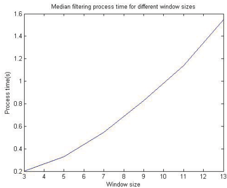
Fig. 21. Computational time against different window sizes.
