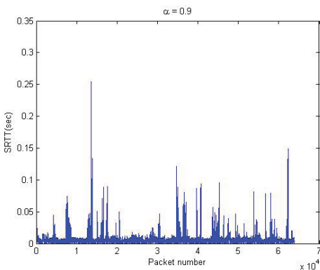
Fig. 6. Smoothed RTT by using (1)
