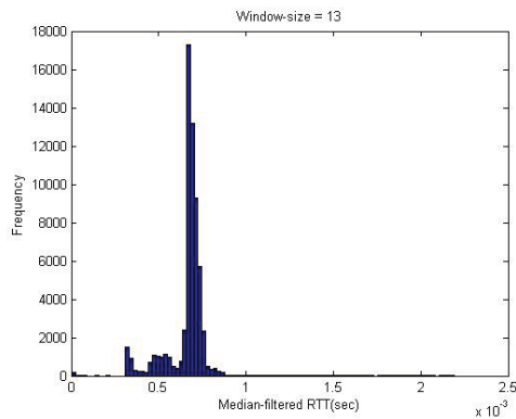
Fig. 20. Histogram of median-filtered RTT with window size equals to thirteen.
