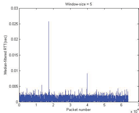
Fig. 3. Median-filtered RTT with window size equal to five.
