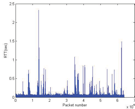
Fig. 1. Unfiltered RTT from a wireless connection.
