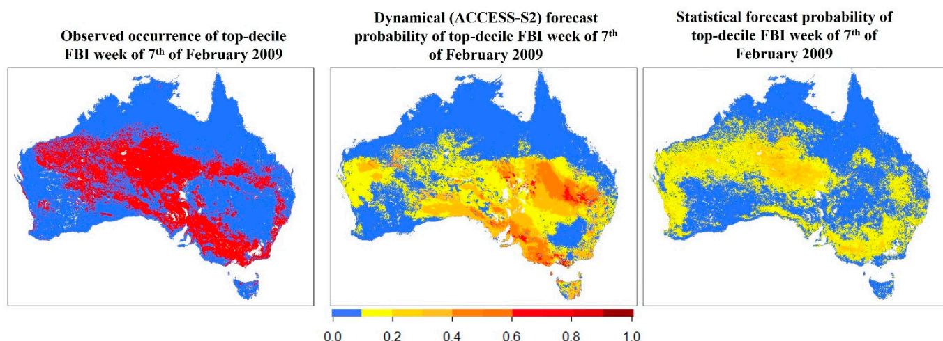
Figure 3. Observed occurrence and forecasted probability of 90th percentile FBI on the week of 7 February 2009.
