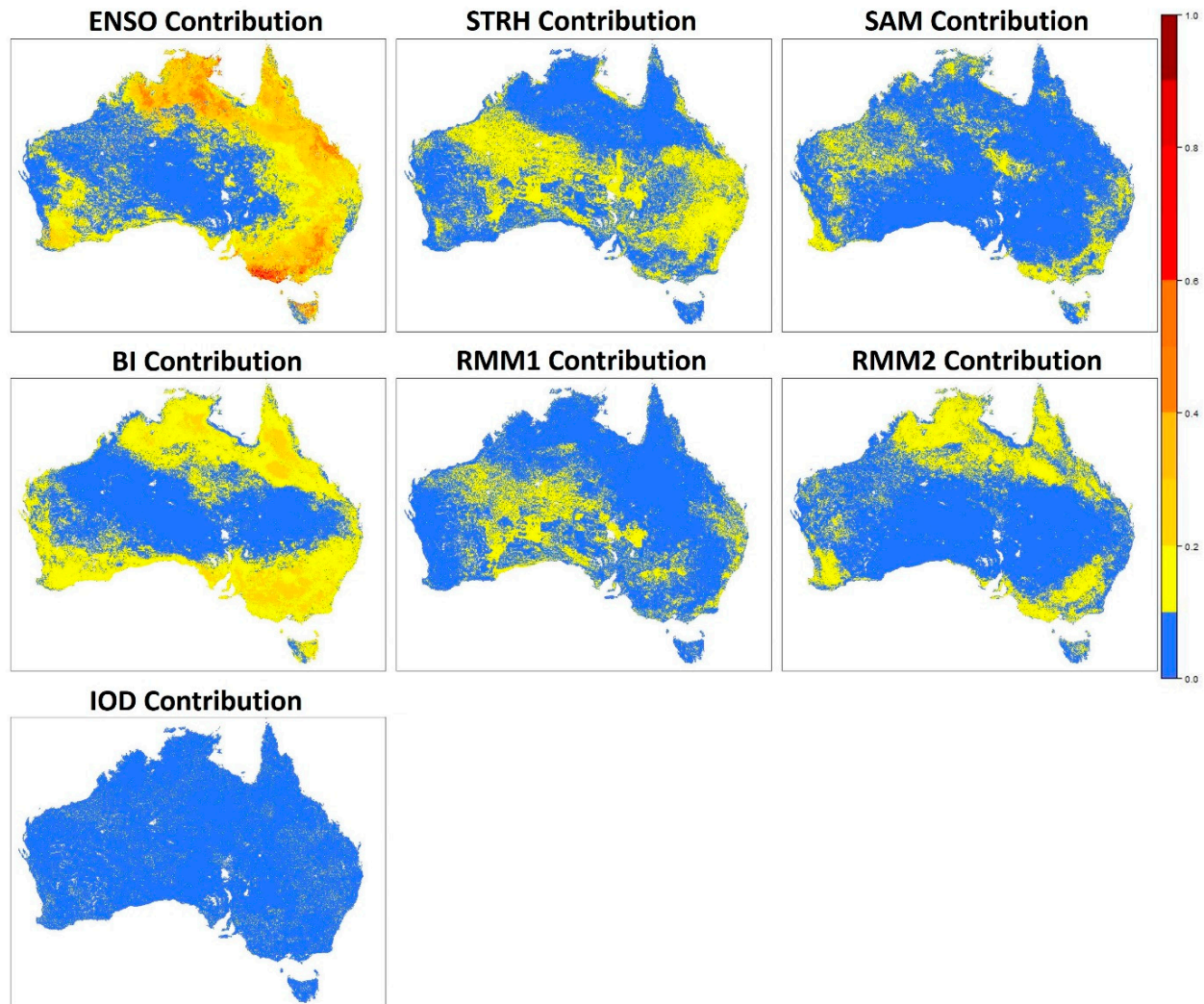
Figure 6. Contribution of each climate driver to statistical forecast probability of 90th percentile FBI for the week of 25 November 2015 according to linear regression.
