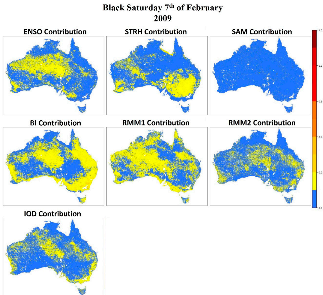
Figure 4. Contribution of each climate driver to statistical forecast probability of 90th percentile FBI for the week of 7 February 2009 according to linear regression.
