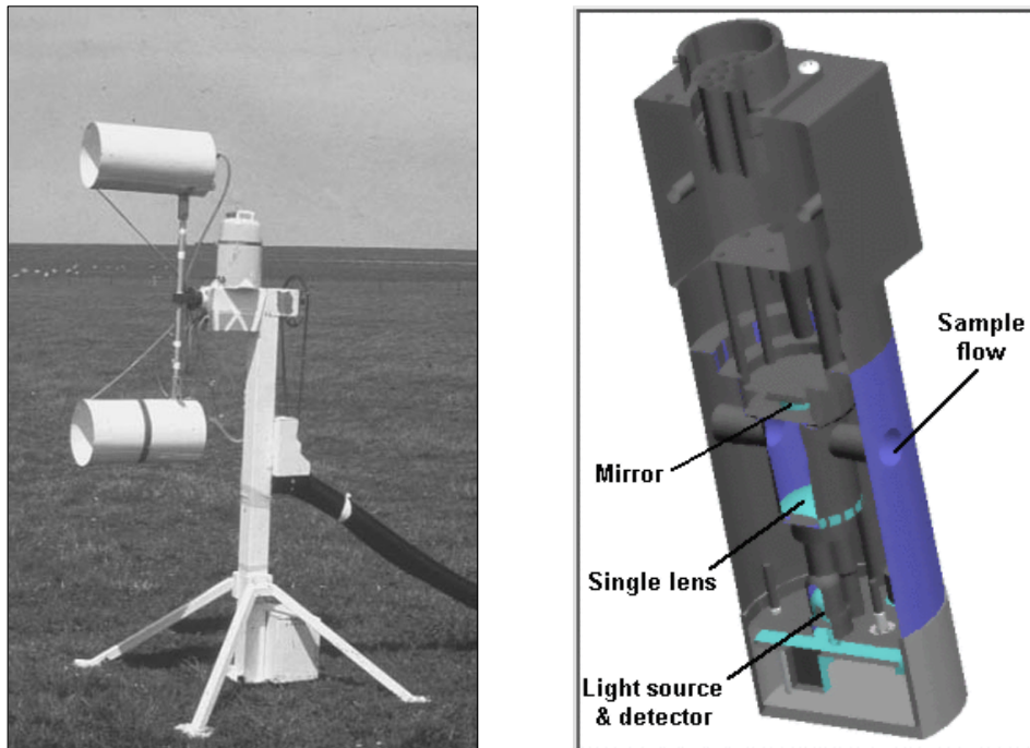
Figure 18: Rotating Arm (paired aspirating psychrometers) and Alternate Flow (cooled mirror hygrometer) units used in accurate Bowen Ratio measurements
