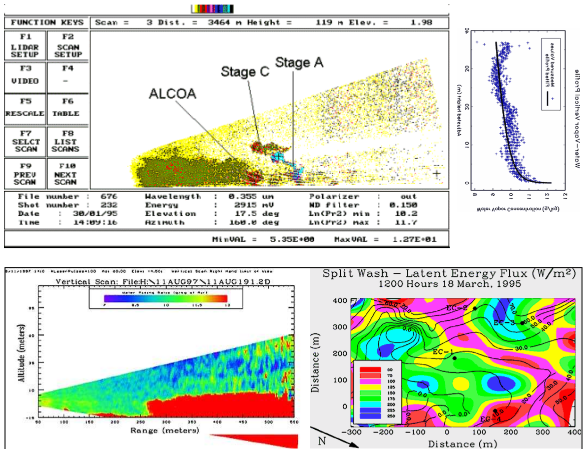
Figure 22: Typical output data from the LIDAR unit
