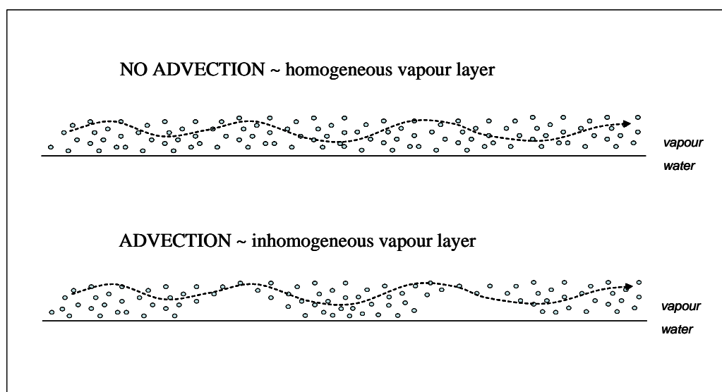
Figure 25: Concept of equilibrium and homogeneity associated with local scale advection
