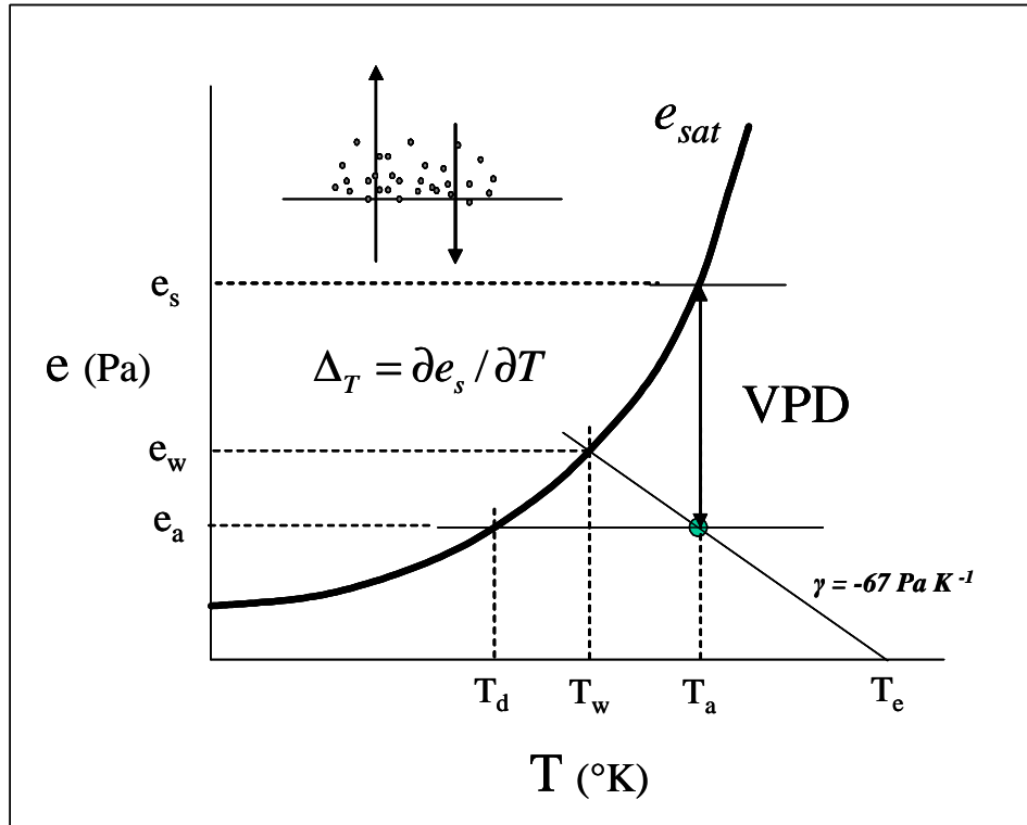
Figure 13: Principle of evaporation
