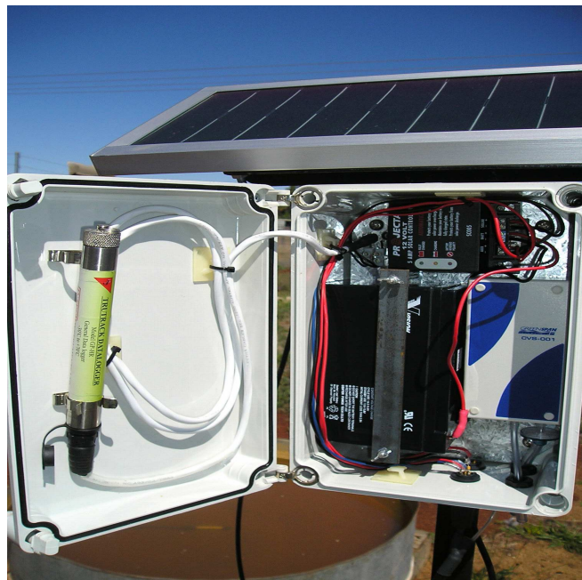
Figure 10: Data logger, solar panel, battery, power management system and PST air breather system
