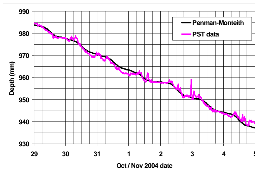
Figure 11: Some typical PST water depth data matched against Penman-Monteith prediction of evaporation
