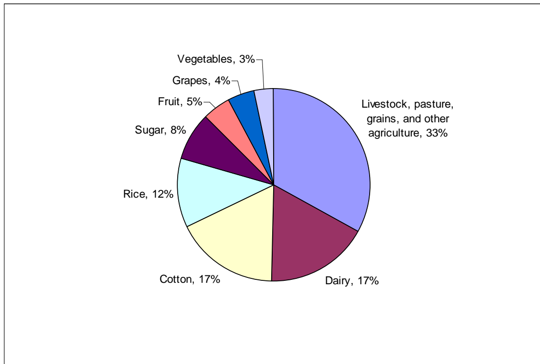
Figure 1: Approximate mean use of agricultural water in Australia (derived from Australian Bureau of Statistics 2001; 2004)
