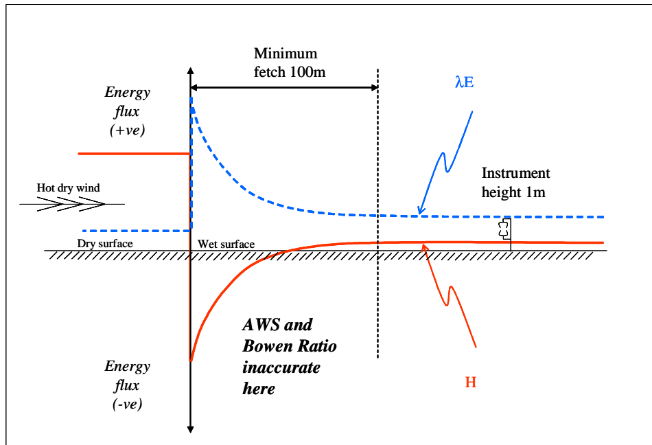
Figure 24: Simplified representation of local advection (after Oke 1987)
