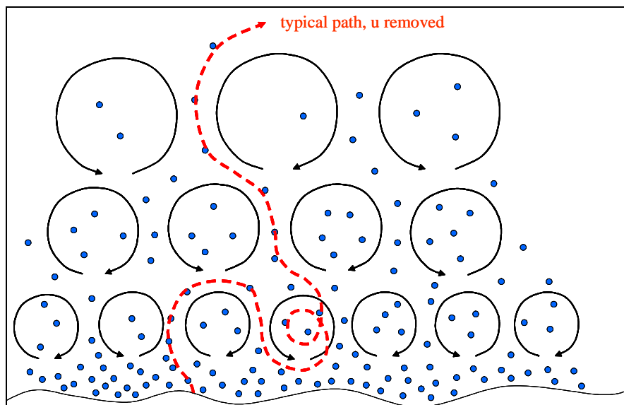
Figure 20: Principle of operation of Eddy Correlation system. The humidity (concentration of water molecules) of upward versus downward moving air is compared to give the humidity flux
