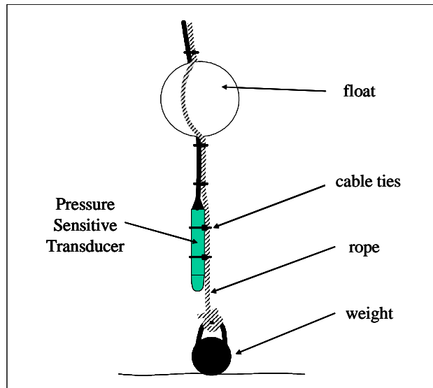
Figure 9: PST installation under the water
