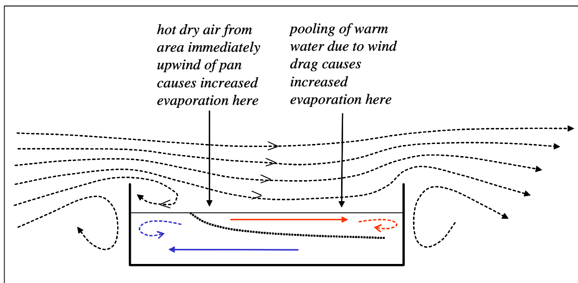
Figure 16: Aerodynamic lip / advective effects associated with evaporation pans
