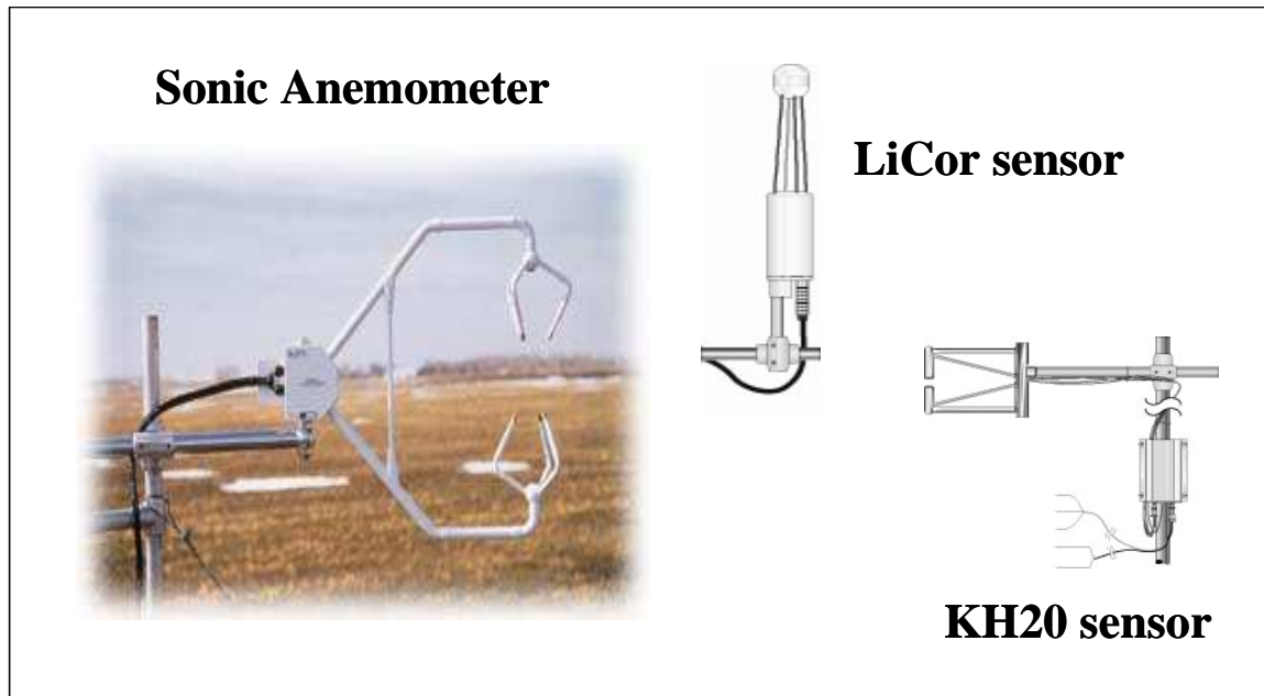
Figure 19: Typical eddy correlation equipment including 3 axis sonic anemometer and LiCor (IR) or KH20 (UV) based fast response humidity sensors (pictures are courtesy of Campbell Scientific Australia)
