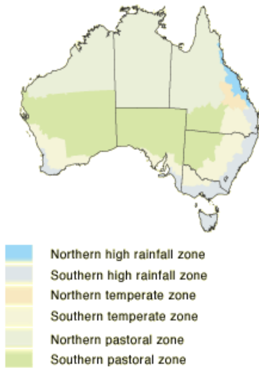
Figure 3: Beef producing regions in Australia
