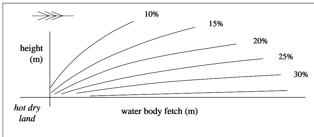
Figure 23: Principle of added evaporation energy due to the oasis effect. Relative Humidity contours predicted by the model of Webster and Sherman (1995) are depressed at the upwind margin of the water body, due to advection of hot dry air from an adjacent land mass.
