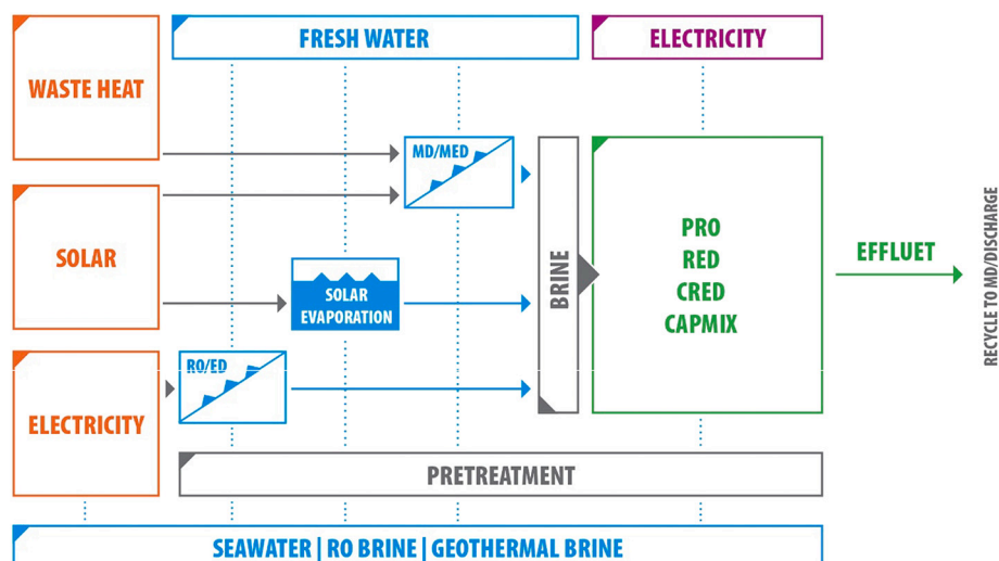
Fig. 3. Concept of simultaneous generation of renewable energy and drinking water production (based on [69] updated).
