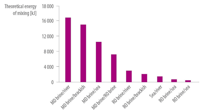
Fig. 4. Theoretical amount of energy (kJ) obtained from different solutions, by mixing 1 \text{ m}^3 of high saline solution and 1 \text{ m}^3 of low mineralized solution (based on [69]).
