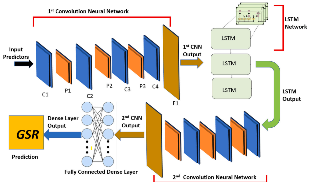
Fig. 5. Architecture of the proposed GSR prediction method based on the hybrid SMA-CNN-LSTM-CNN-MLP (SCLC) model.
