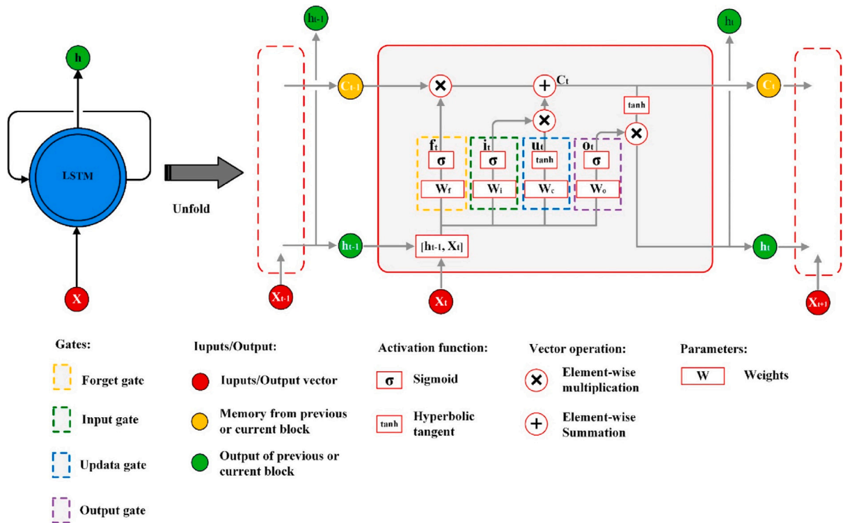
Fig. 4. The structure of Long-Short Term Memory (LSTM) Network.
