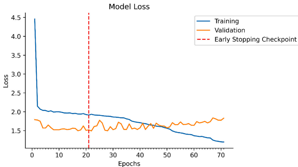
Fig. 9. Losses (training and validation with mean absolute error) for the prediction of GSR. Absence of loss improvement with predefined epochs calls for the early stopping callbacks.
