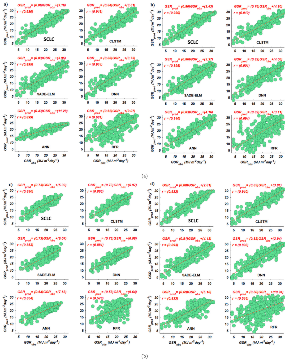
Fig. 11. Scatter plots of predicted (GSR pred ) and observed (GSR obs ) for all tested regions in Six solar farms of Queensland. (a) Barunggam, (b) Cameby Solar Farm, (c) Cape York Solar Storage, (d) Chinchilla, (e) Clermont and (f) Sun Metals. (Note: Red line is the least-squares fit line ( y = mx + c ). Table 3 as well as Tables 4 and 5) show the model nomenclature.
