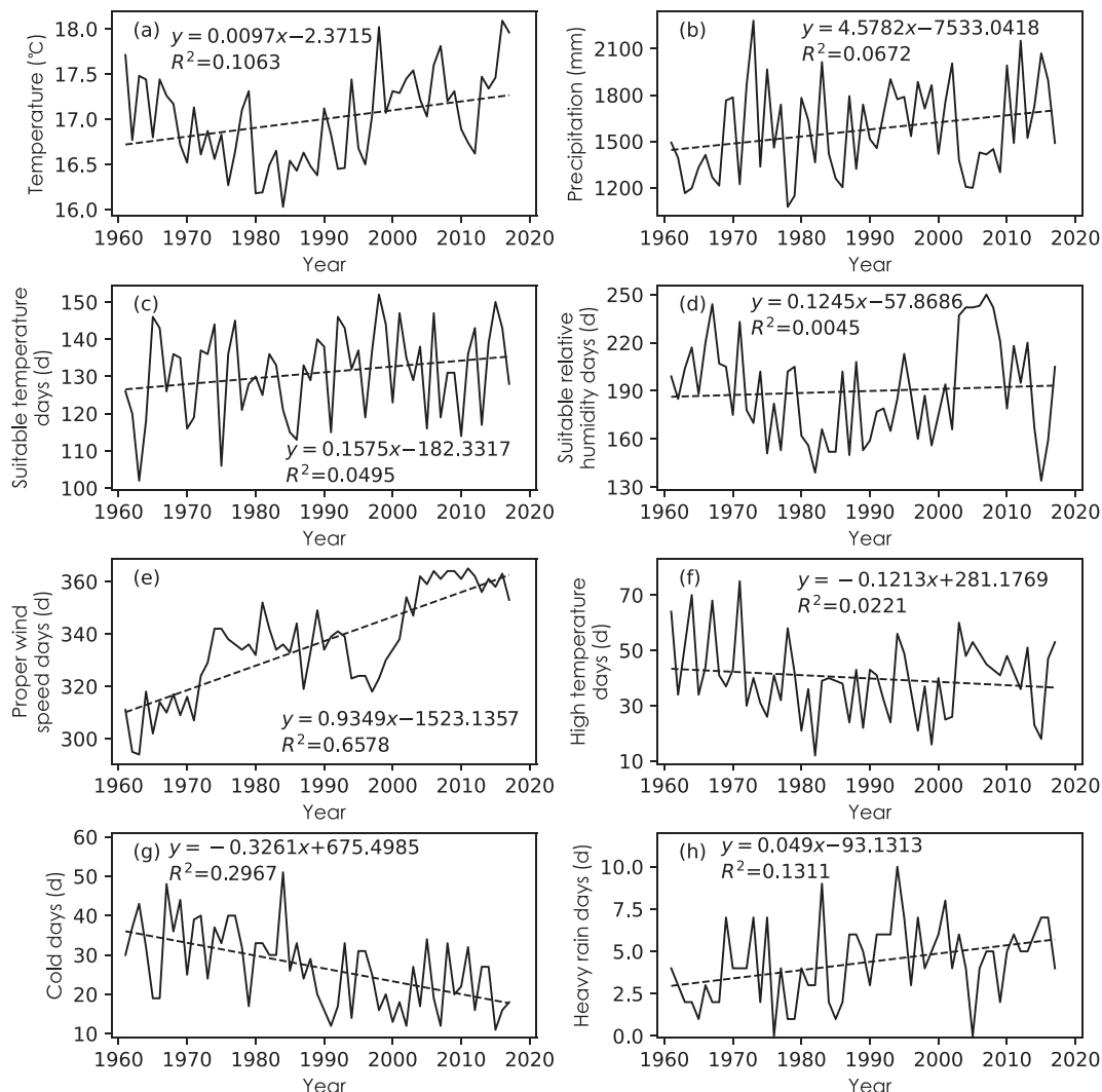
Fig. 3. Changes of climate elements and the linear trends in Jiande city, Zhejiang province from 1961 to 2017.
