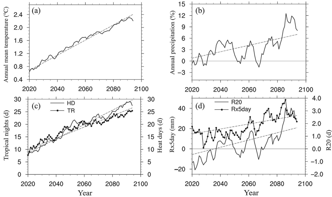
Fig. 4. Projected changes in the area averaged annual (a) mean temperature, (b) precipitation, (c) tropical nights (TR) and heat days (HD), and (d) R20 and Rx5day (The values are smoothed by a 9-year running mean; the dash lines indicate linear trends).
