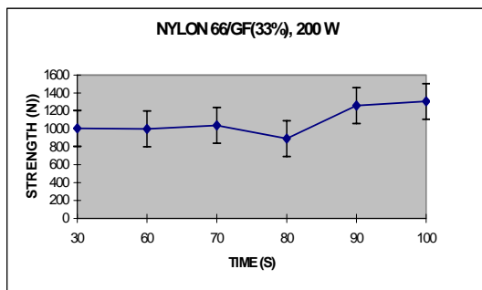
Figure 5: Bond Strength of Nylon 66/GF (33%) with Araldite Using VMF
