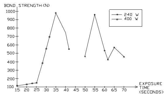
Figure 6: Bond Strength of Nylon 66/GF (33%) with Araldite Using FFM
