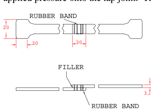
Figure 3: Two Mirror Image Test Pieces of Nylon 66/GF (33%)
