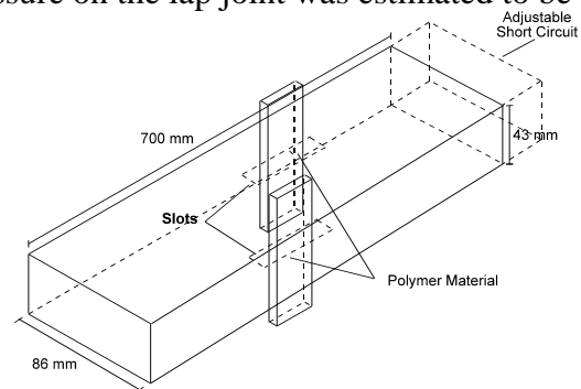
Figure 4: Slotted Waveguide Used for Joining Nylon 66/ GF (33%) Using Rapid Araldite
