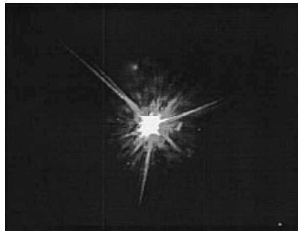
FIG. 4. Centered 256 grayscale reference image (clear sky, 1159 LT 9 Sep 1997), 200 × 320 pixels.
