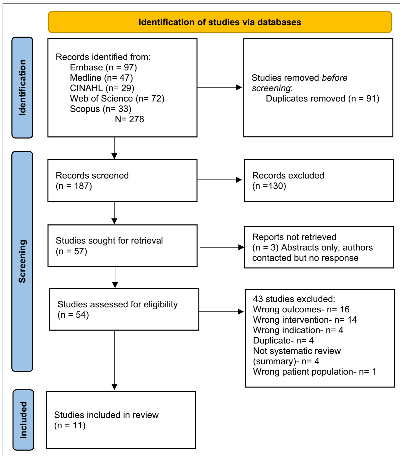
Figure 1. PRISMA.
