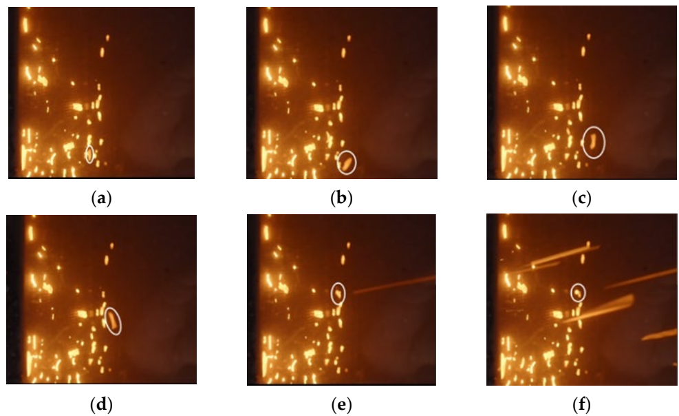
Figure 13. Firebrands bounce back after hitting the mesh. The encircled firebrands (a) impact the mesh, (b) bounce back, (c–e) return to the mesh and (f) settle into a new position and continue to burn (Stainless Steel Wire and Mesh Pty Ltd. [17]).
