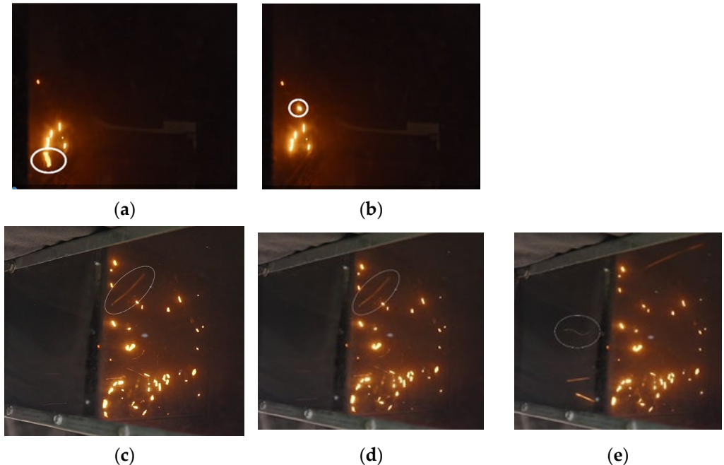
Figure 14. The slipping firebrands, (a) a firebrand at hitting point, (b) the firebrand slipped and changed and became a pausing firebrand, (c) an approaching firebrand, (d) the slippage of the firebrand, (e) the firebrand became quenched at its new location and passed (stopping firebrand) (Stainless Steel Wire and Mesh Pty Ltd. [17]).
