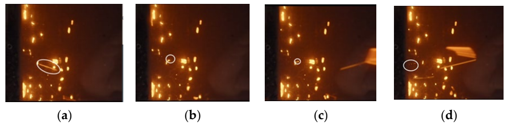
Figure 12. Firebrands continue to burn before penetrating the mesh, (a) approaching the firebrand, (b) stopping stationary at the hitting point, (c) continuation of burning and fragmentation into two smaller firebrands, and (d) penetrating the mesh (Stainless Steel Wire and Mesh Pty Ltd. [17]).
