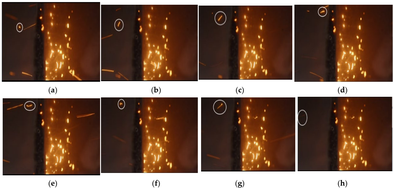
Figure 15. Wandering of small firebrands at the exit side of the mesh in consecutive frames of (a–g) shows the end of wandering and movement in wind direction, (h) shows the firebrand quenched (Stainless Steel Wire and Mesh Pty Ltd. [17]).
