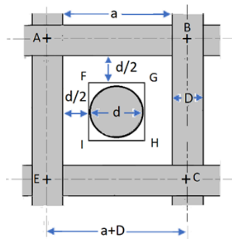
Figure 19. Passage of firebrand with a diameter d through a screen with wire diameter D and aperture a .
